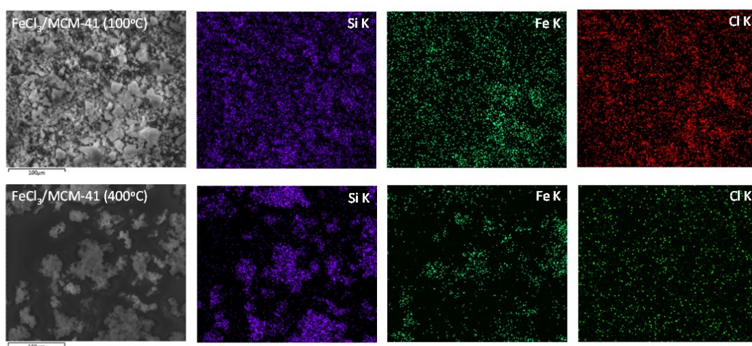
Figure S1: SEM-EDX Mapping of FeCl 3 /MCM-41 dried at 100 °C (upper panel) and calcined at 400 °C (lower panel)
