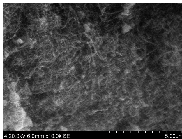
Figure S1 the magnified SEM images of untreated MWCNT-COOH
