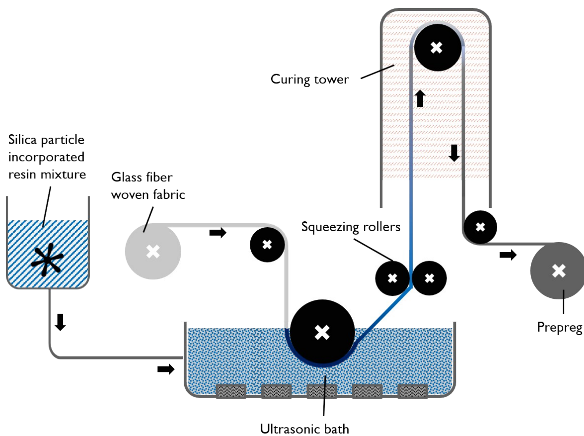
Figure S1. Schematic illustration of ultrasonic induced solvent impregnation process of silica bead incorporated epoxy/glass fibre prepreg.
