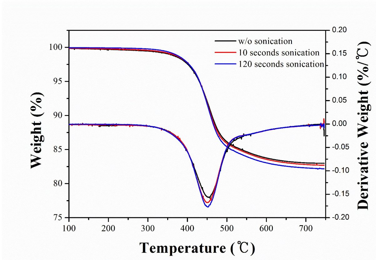
Figure S2. TGA curves of epoxy/glass fibre/bead composite laminate specimens w/o sonication, 10 sec sonication, and 120 sec sonication presenting similar residual weight.
