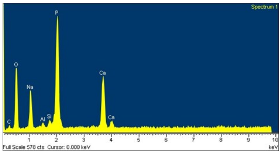
Fig S4. EDX pattern of DIPH.
