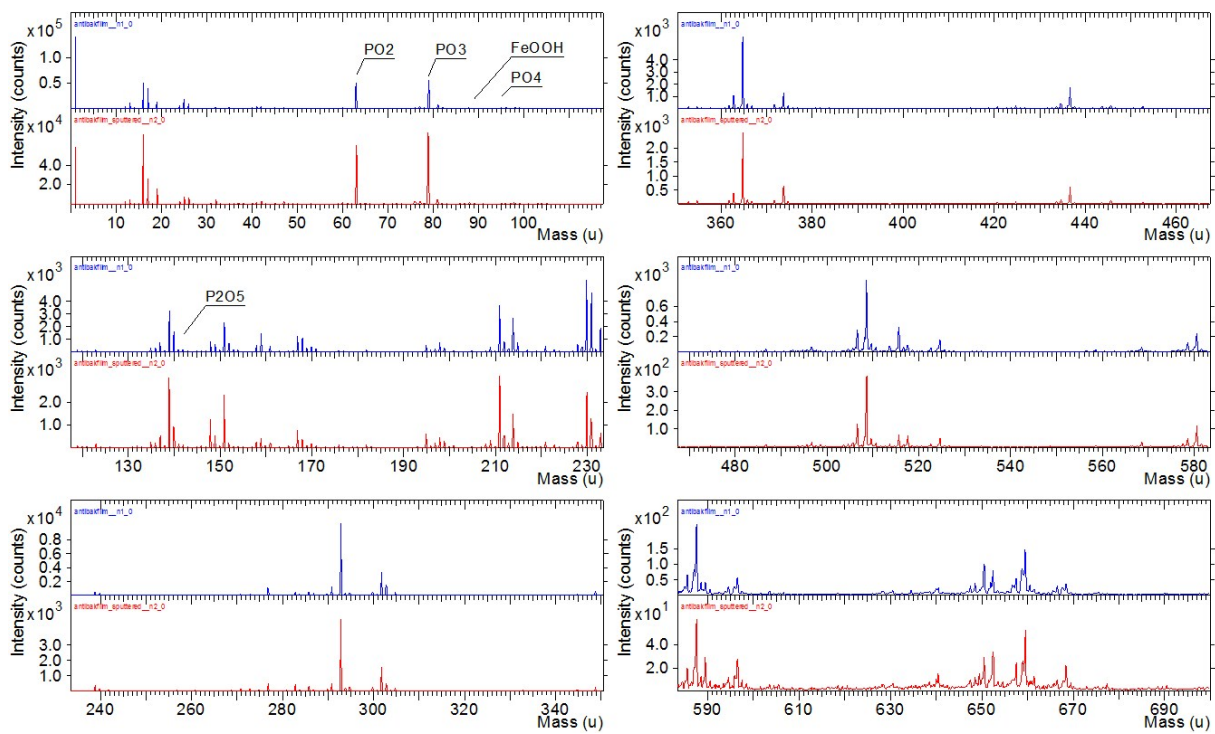
Mass spectrometry (TOF-MS) of negatively charged ions on the surface of FeO x -PO x -HDPET
