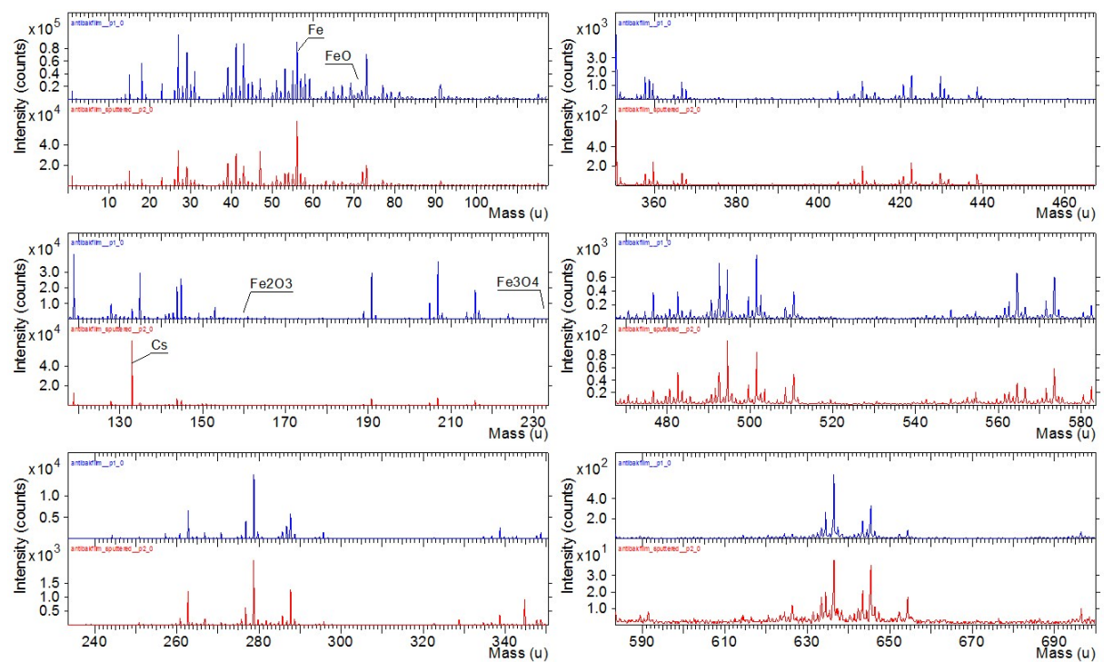
S2: Mass spectrometry (TOF-MS) of positively charged ions on the surface of FeO x -PO x -HDPET
