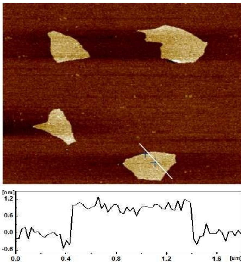
Fig. S1 A typical AFM image of GO sheets deposited onto a mica substrate from an aqueous dispersion.
