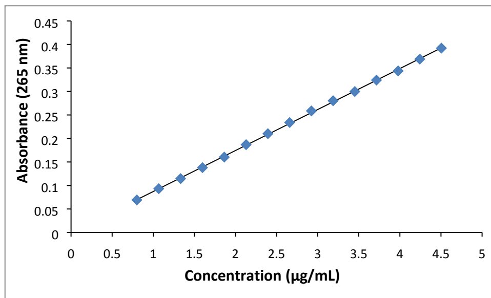
Fig. S1. The calibration curve of AZT at 265 nm.
