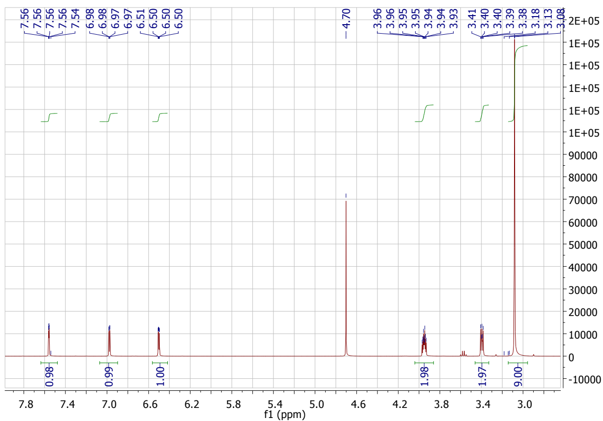
Figure f: 1 H NMR spectrum of [Chol][Fur] (with residual ethanol)
