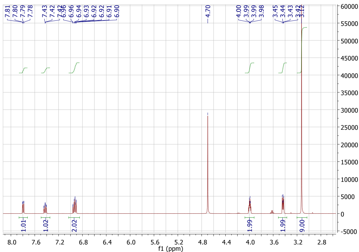
Figure c: ^1\text{H} NMR spectrum of [Chol][Sal] (with residual ethanol)
