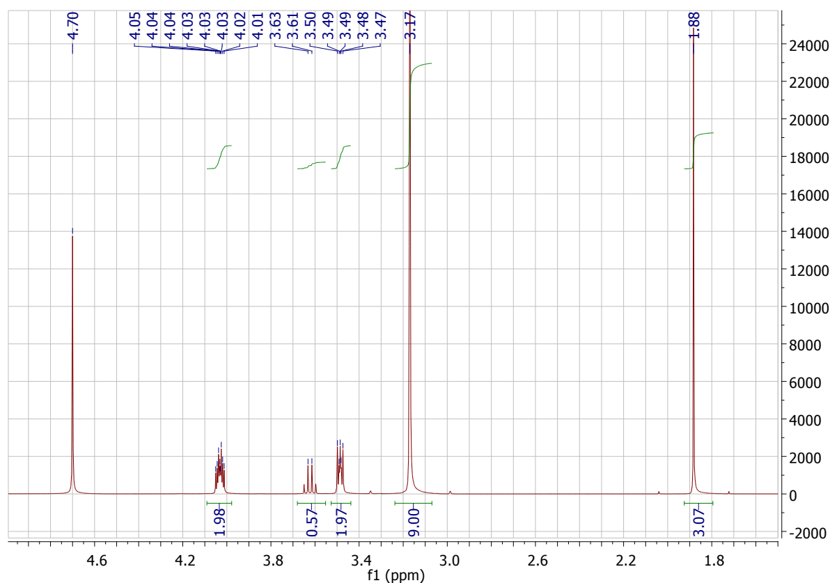
Figure a: 1 H NMR spectrum of [Chol][Ace] (with residual ethanol)
