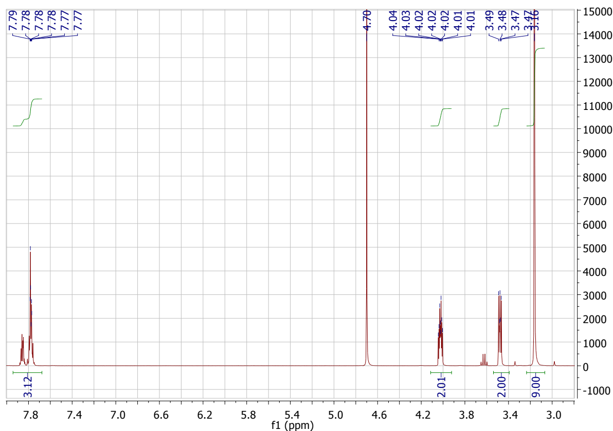
Figure b: 1 H NMR spectrum of [Chol][Sac] (with residual ethanol)
