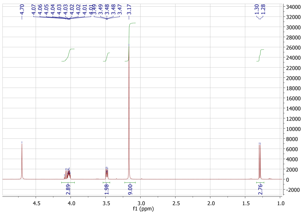
Figure e: 1 H NMR spectrum of [Chol][Lac]
