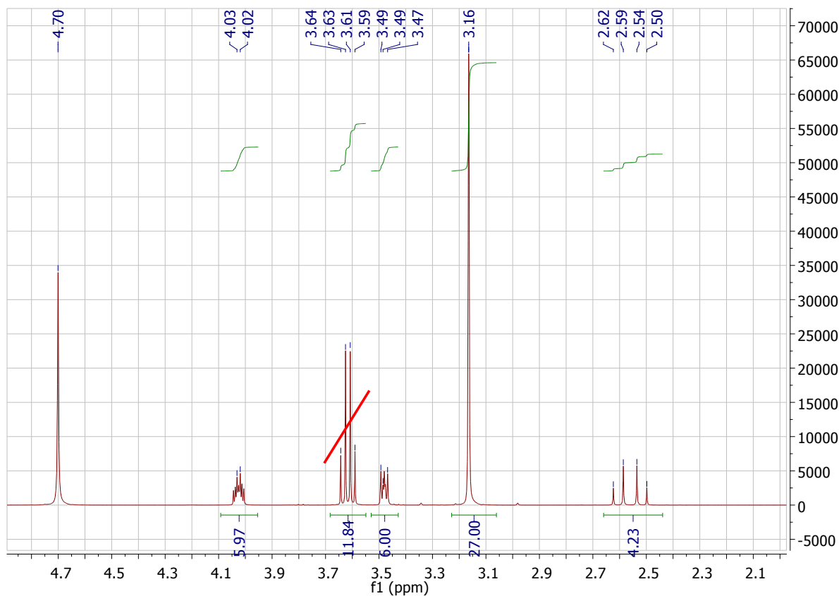
Figure d: ^1\text{H} NMR spectrum of [Chol][Cit] (with residual ethanol)
