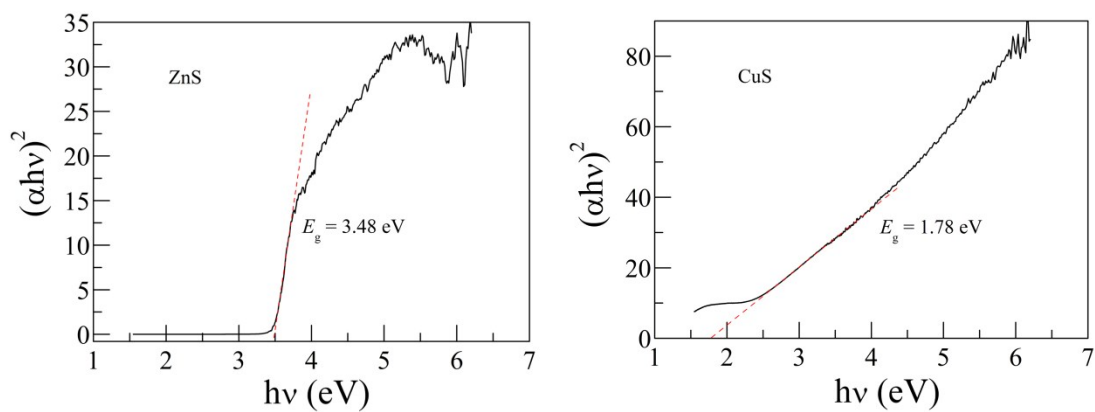
Fig. S1 Tauc plot of ZnS and CuS.
