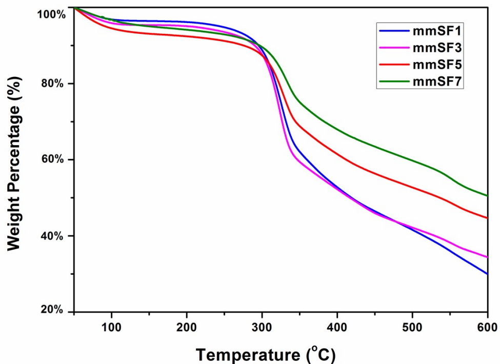
Fig.S1 TGA curves of mineralized silk microfibers for different periods: 1 day, mmSF1; 3 days, mmSF3; 5 days, mmSF5; 7 days, mmSF7.
