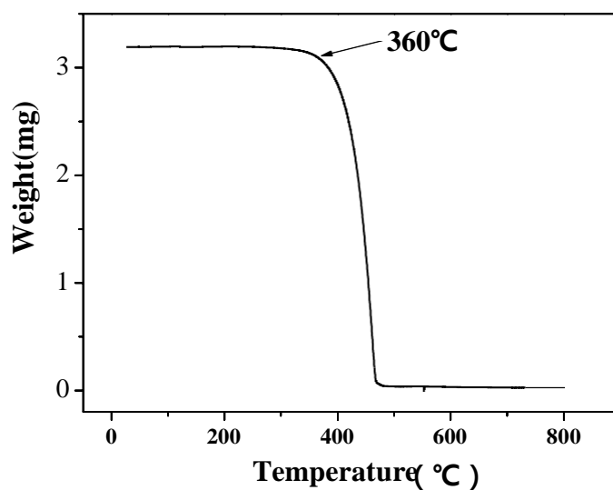
Supplementary Figure 1 The TGA curve of PDI-i8C compound
