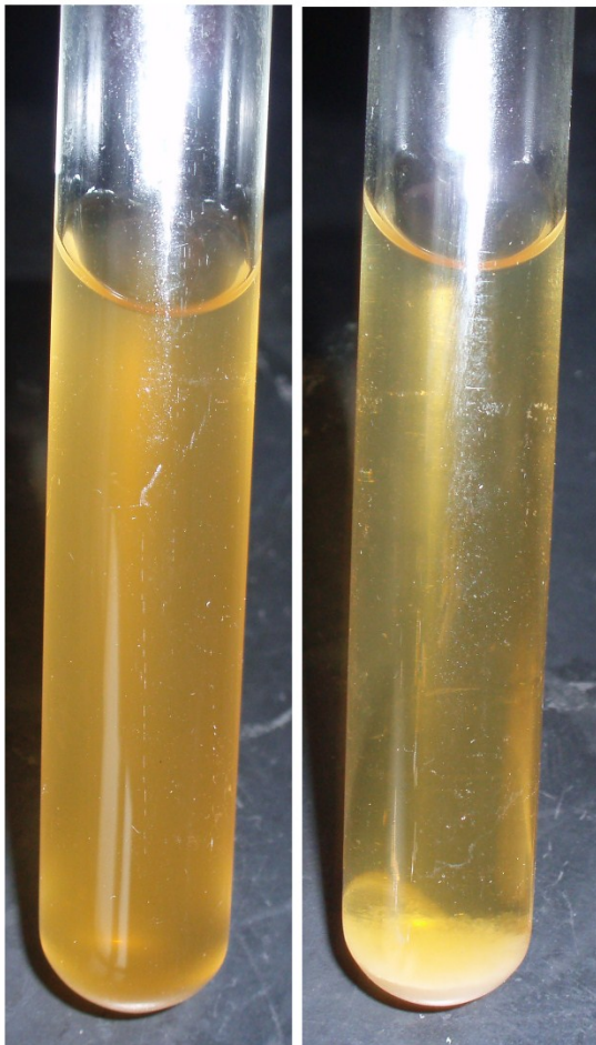
Figure S3 Lipopeptides produced by Bacillus flexus S1 fed with LB medium. Left picture is pure LB medium as control test. Right picture is LB medium cultured with Bacillus flexus S1, and the white precipitates in the bottom of cuvette is lipopeptides.
