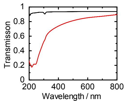
Figure S2 UV-vis transmission spectra of pDDA nanosheets (9)/HKUST-1(10) deposited on a CaF 2 plate (red) and bare CaF 2 plate (black).
