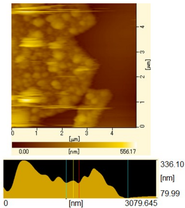
Figure S1 (Top) Surface topography image of pDDA(9)/HKUST-1(40). (Bottom) Cross-section profile of pDDA(9)/HKUST-1(40).
