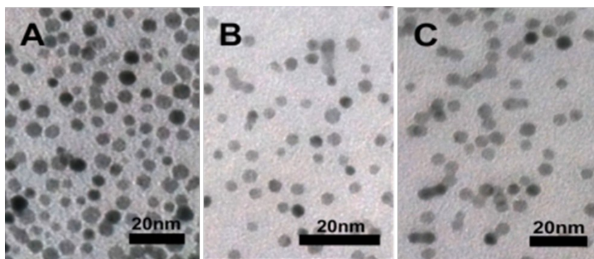
Figure S1 TEM images of Pd intermediates during the synthesis of Pd-a with the reaction time of 30 min (A), 60 min (B) and 120 min (C).
