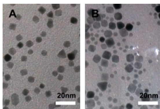
Figure S2 TEM images of Pd products obtained from the systems containing Pd-a as the seed (3 reaction cycles) (A) and solid Pd-b as the seed (B).
