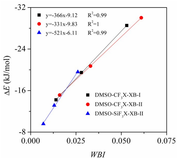
Fig. S2 WBI of O...X halogen bond versus the interaction energy.
