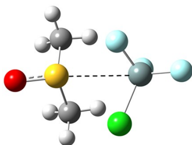
Fig. S1 Optimized structure of S...Si bonded complex of DMSO-SiF 3 Cl.
