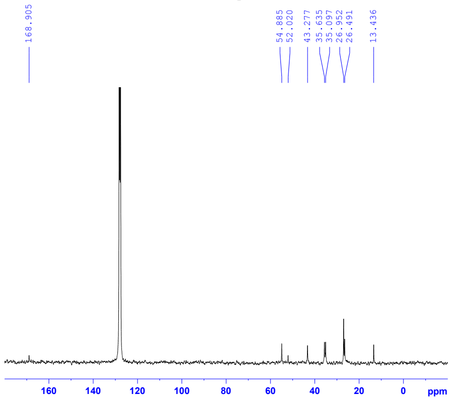
The ^{13}\text{C} NMR spectra of 4
