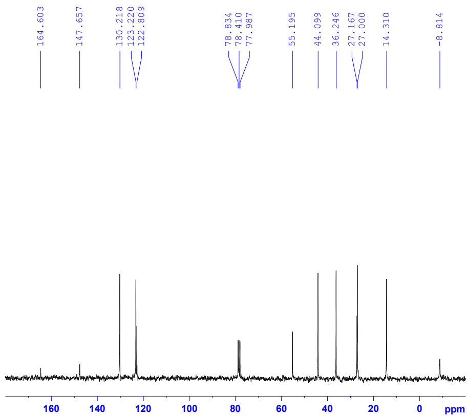
The ^{13}\text{C} NMR spectra of 2
