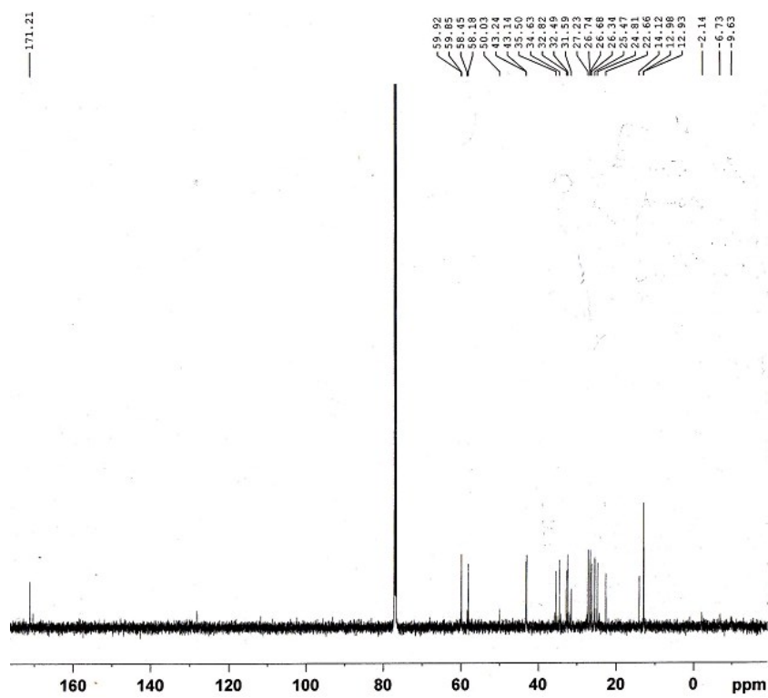
The ^{13}\text{C} NMR spectra of 8
