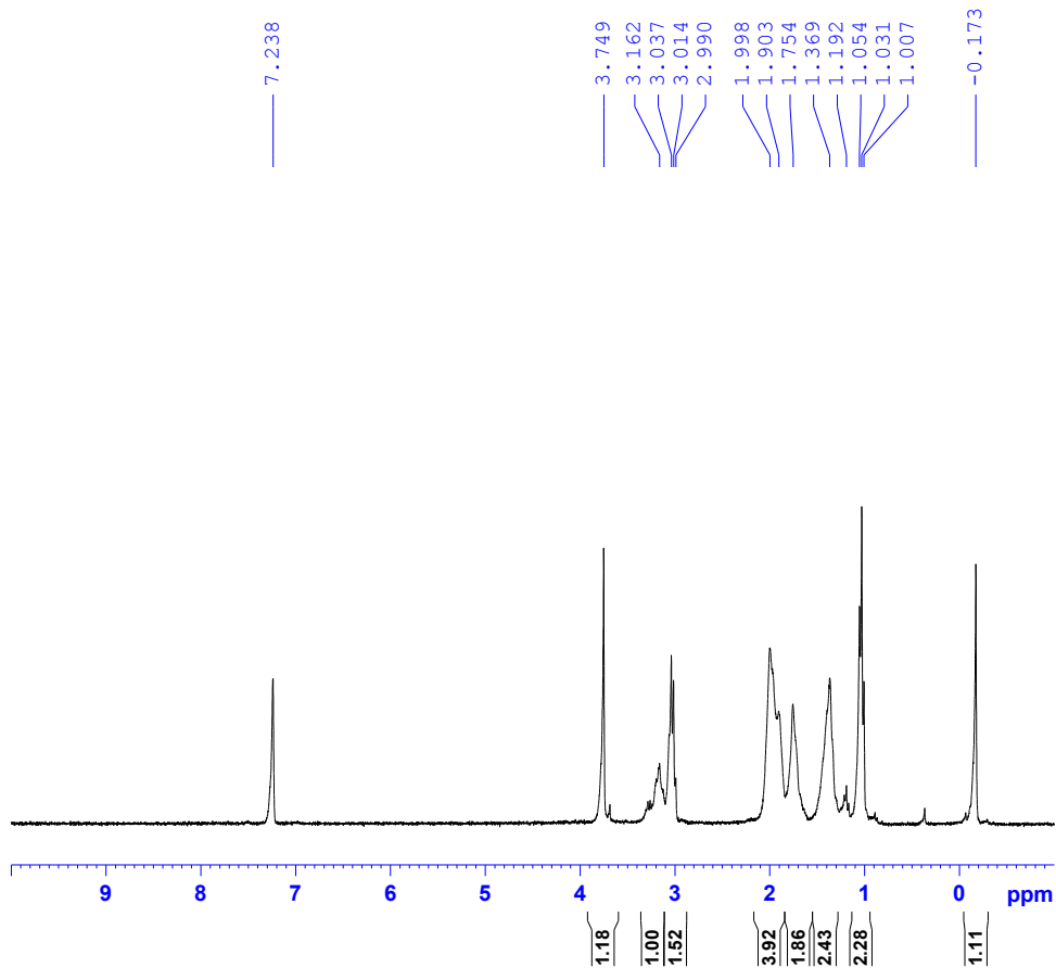
The ^1\text{H} NMR spectra of 4
