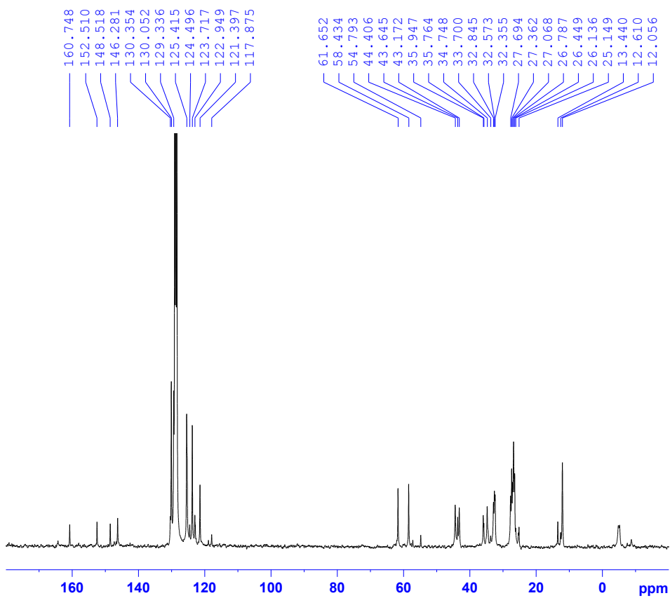
The ^{13}\text{C} NMR spectra of 5
