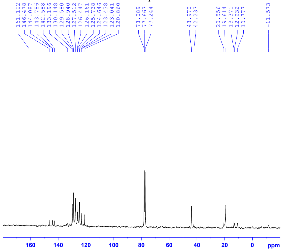
The ^{13}\text{C} NMR spectra of 7
