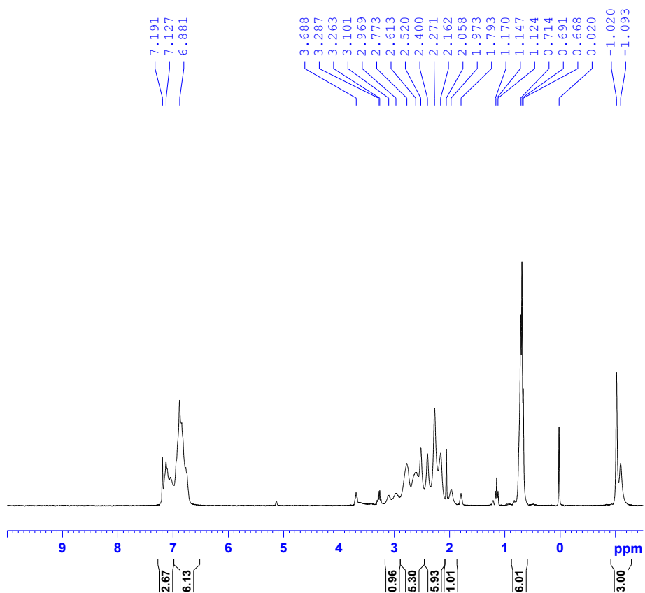
The ^1\text{H} NMR spectra of 6
