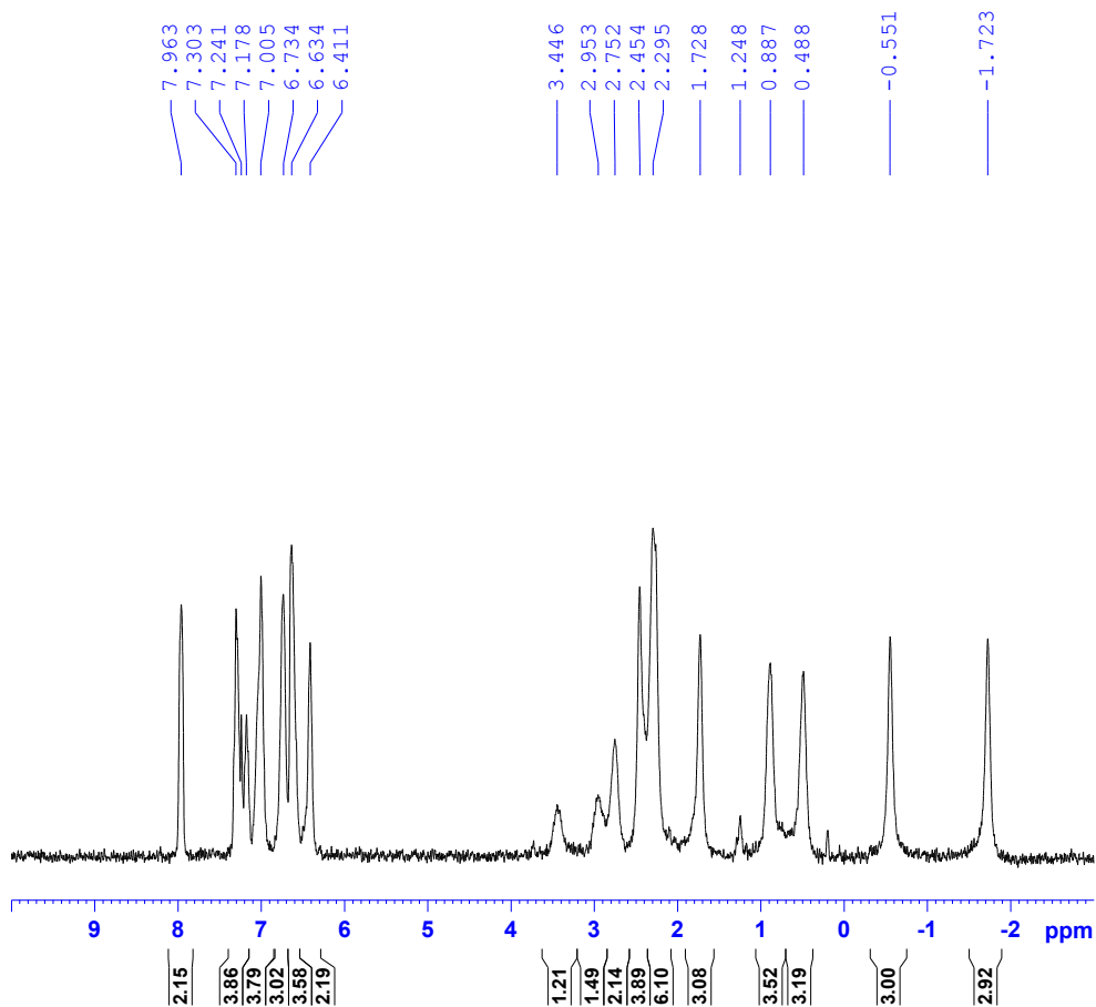
The ^1\text{H} NMR spectra of 7
