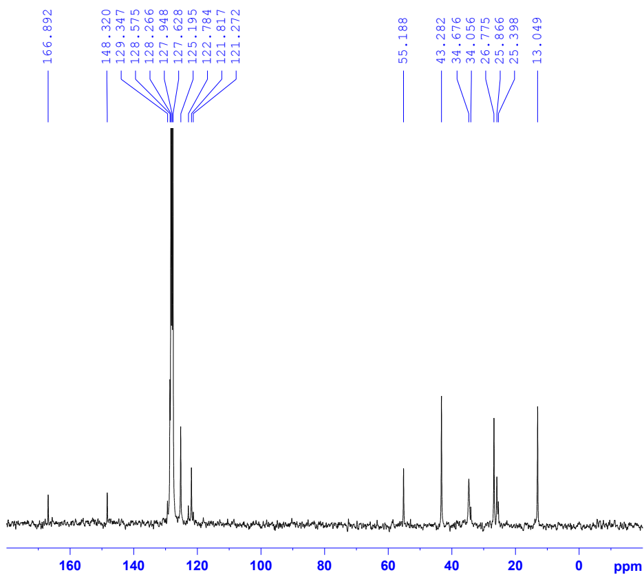
The ^{13}\text{C} NMR spectra of 3
