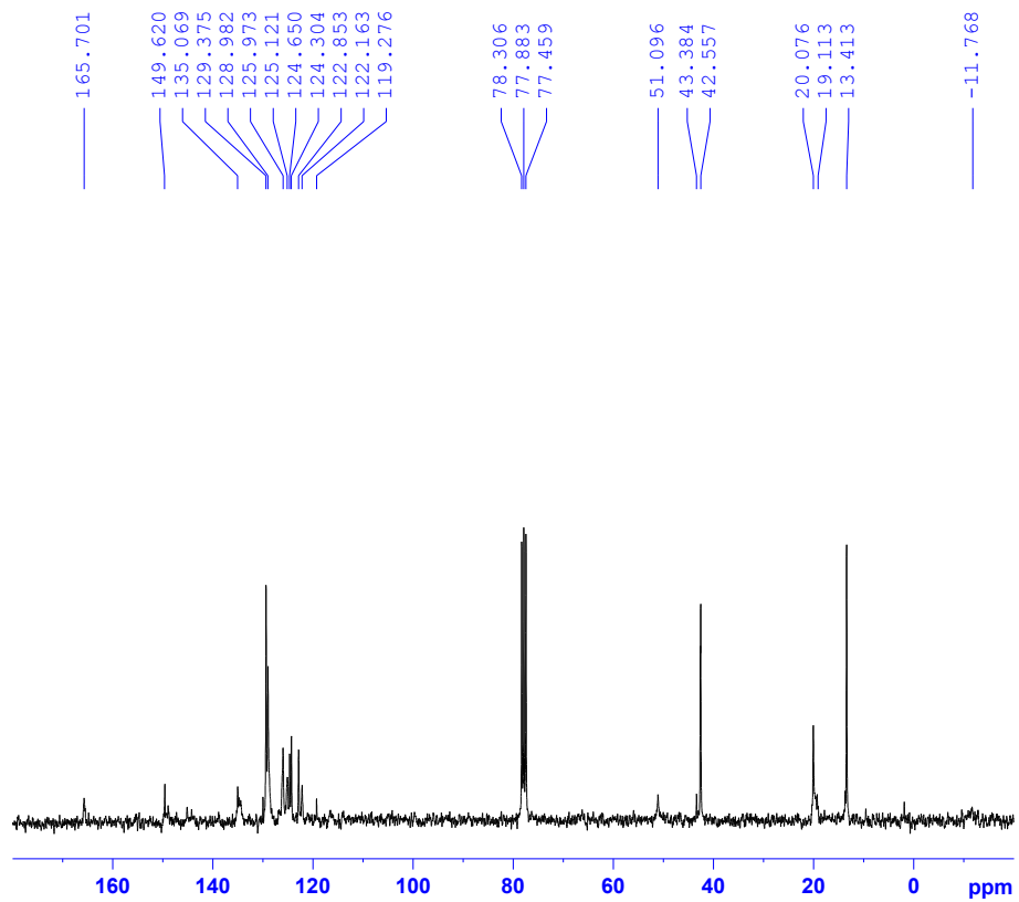
The ^{13}\text{C} NMR spectra of 6
