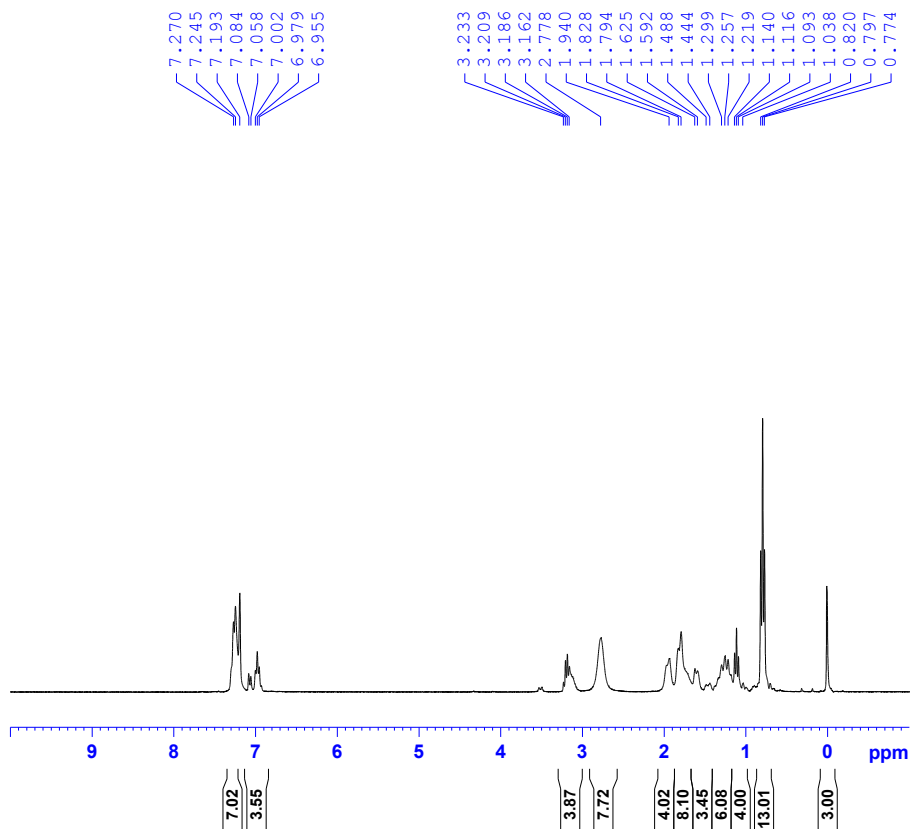
The ^1\text{H} NMR spectra of 3
