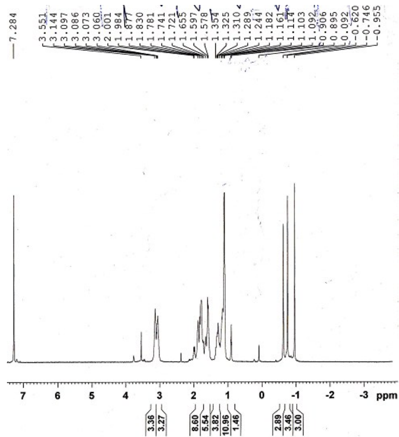
The ^1\text{H} NMR spectra of 8
