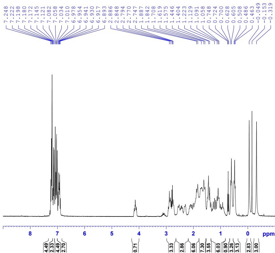
The ^1\text{H} NMR spectra of 5
