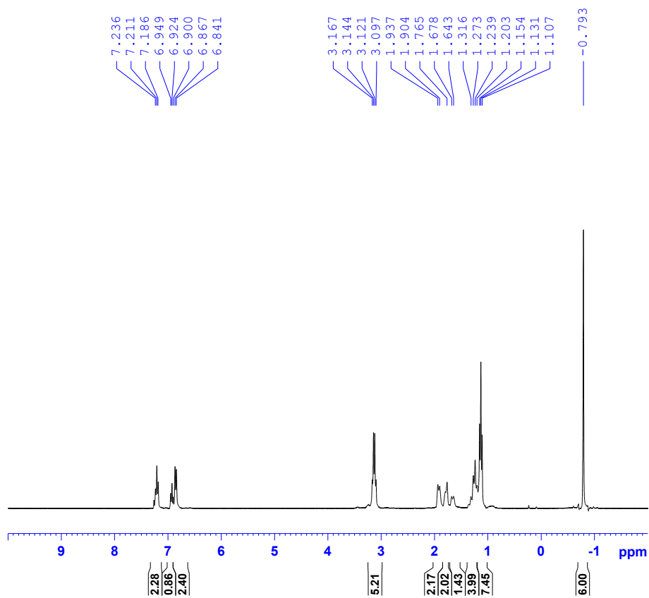
The ^1\text{H} NMR spectra of 2
