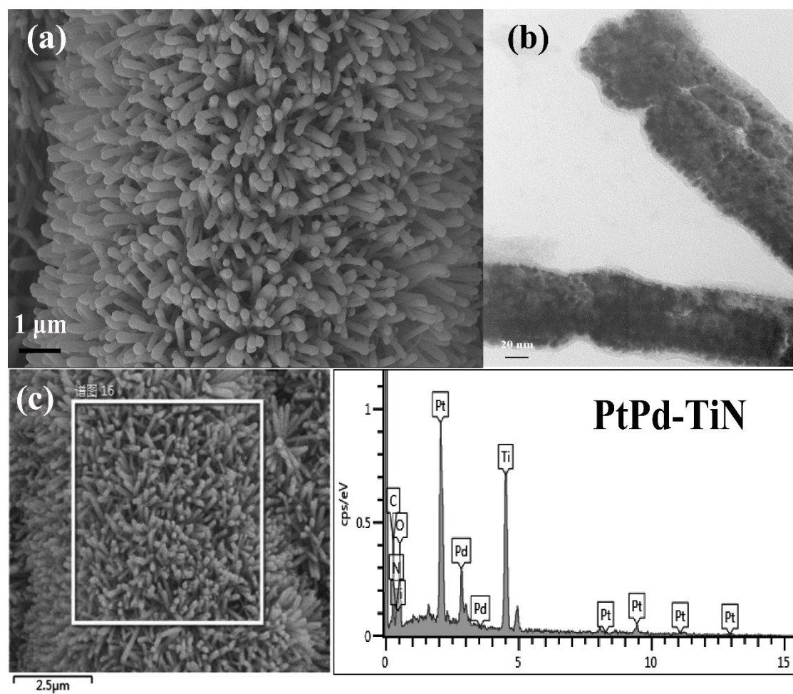
Fig. S1 FESEM image (a), TEM image (b), and EDX (c) of PtPd-TiN NRs
