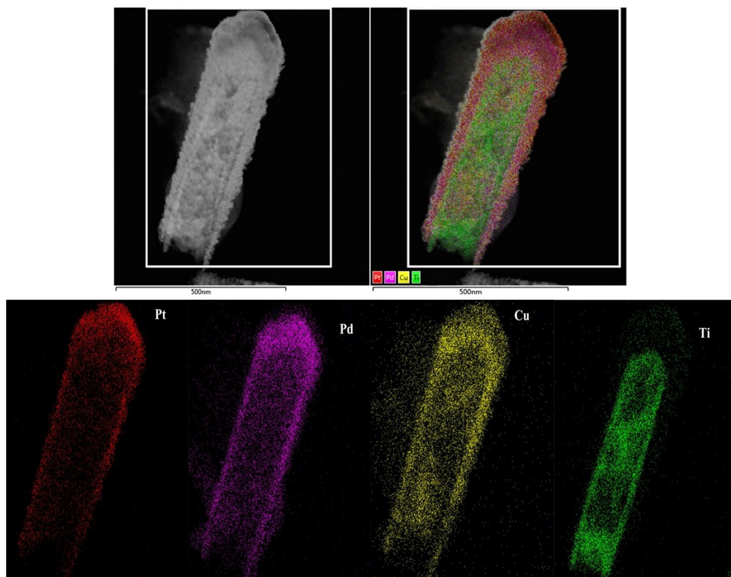
Fig. S2 HAADF-STEM characterization and elemental mapping of a PtPdCu-TiN NR.
