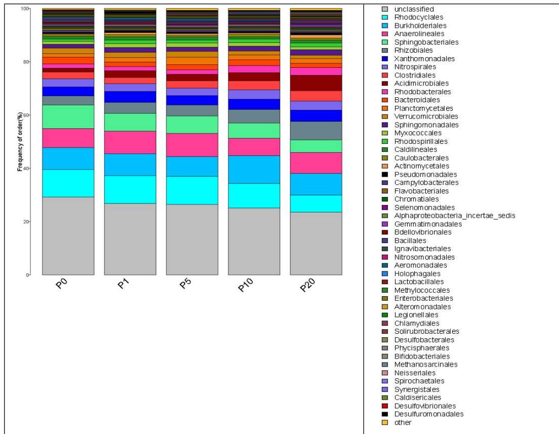
Fig.S4 Flora abundance at the order level in the activated sludge
