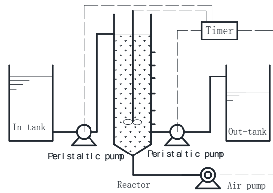
Fig. S1. The setup of sequencing batch reactor (SBR)
