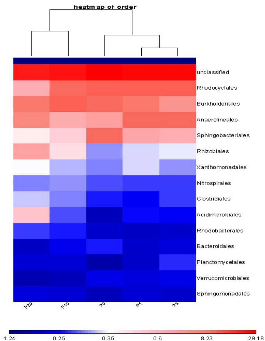
Fig.S3 Species distribution heatmap at the order level in the activated sludge
