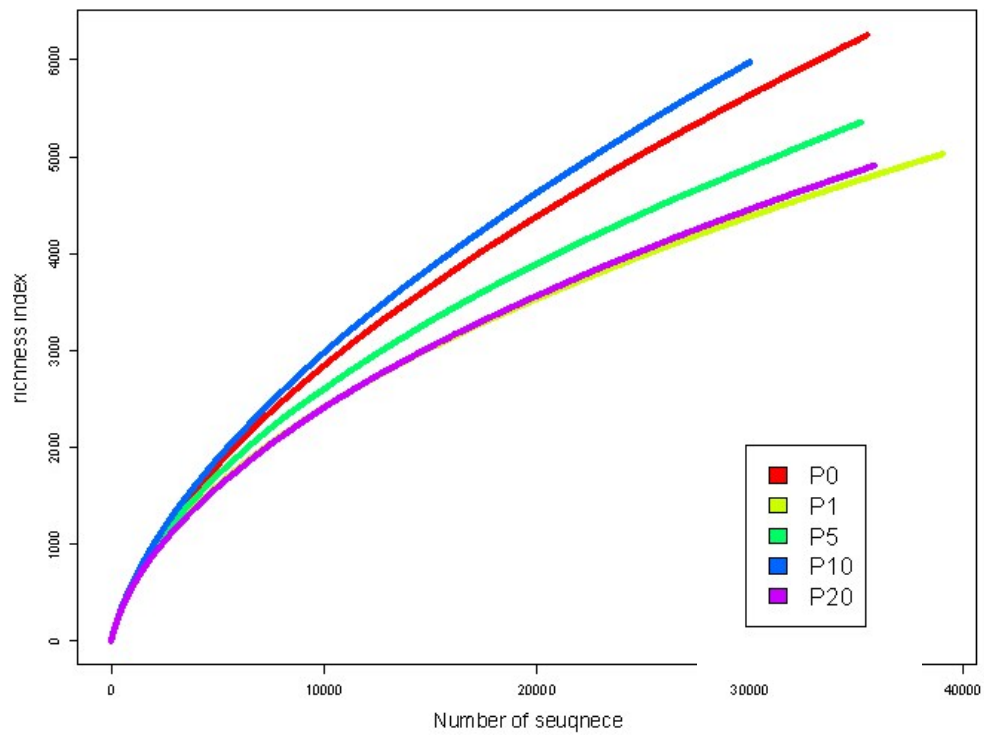
Fig.S2 Richness rarefaction plot of species in the activated sludge
