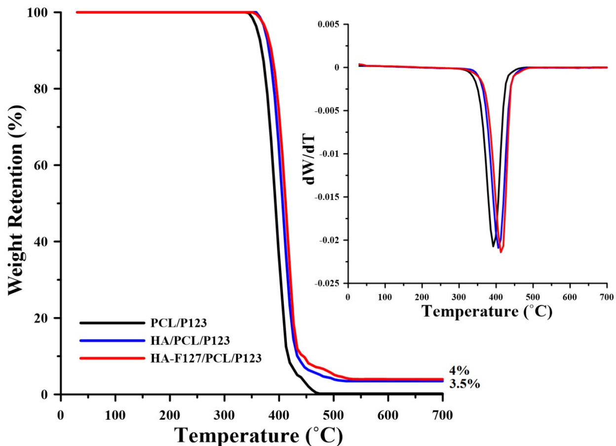
Supplementary Figure 1: TGA and dTG curves of PCL/P123, HA/PCL/P123 and HA-F127/PCL/P123
