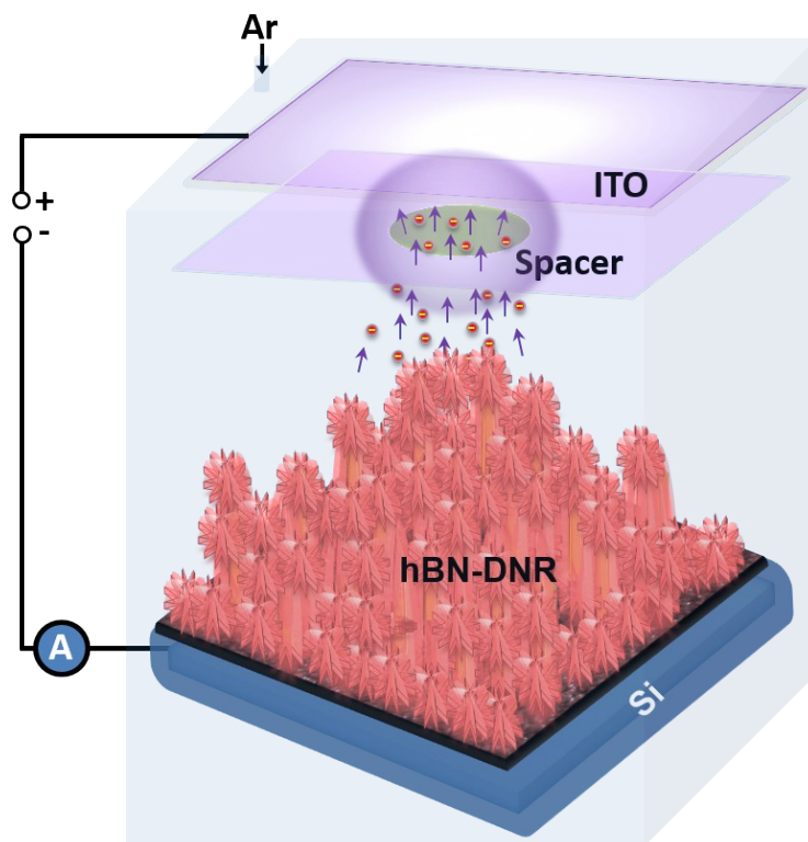
Fig. S2. The schematic of microplasma device measurement.
