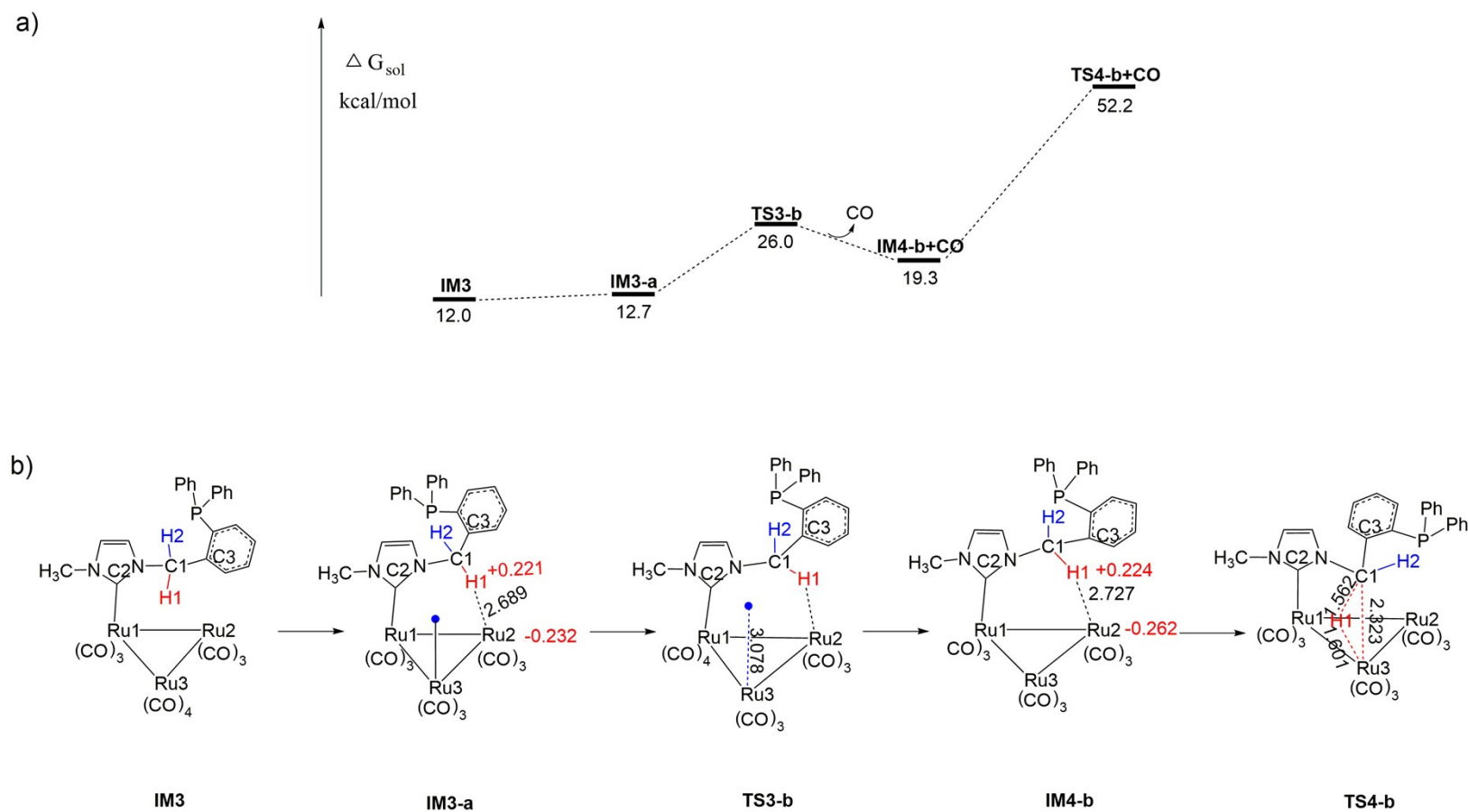
Fig. S2 Calculated free energy profile (a) and the schematic diagrams for the oxidative addition of C1–H1 bond on Ru3 (b). The blue point denotes the CO that will be released from the metal center. Bond lengths in angstroms.
