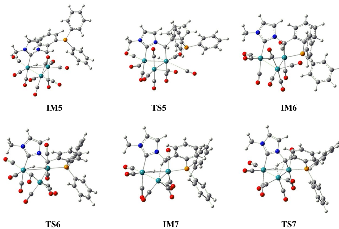
Fig. S4 Optimized geometries for the species shown in Fig. 2.
