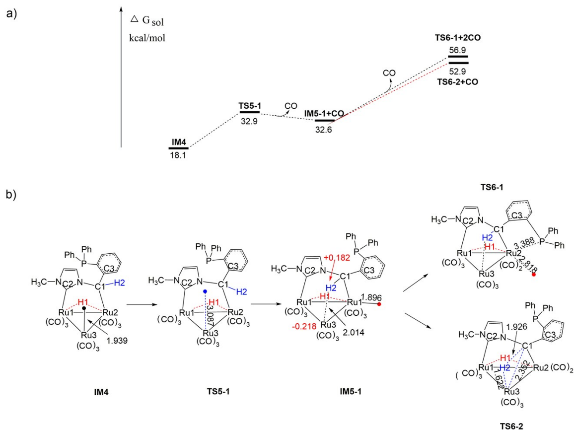
Fig. S6 Calculated free energy profile (a) and the schematic diagrams of the alternative pathways for the second C–H bond activation (b). The red and blue points denote the CO that will be released or is being released from the metal center. Bond lengths in angstroms.
