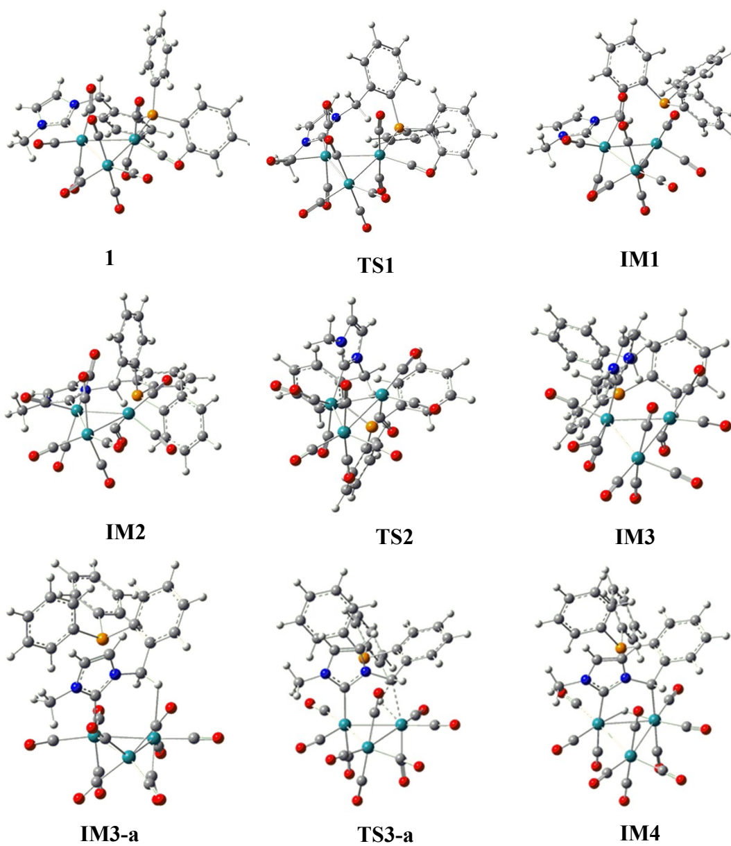
Fig. S1 Optimized geometries for the species shown in Fig.1.
