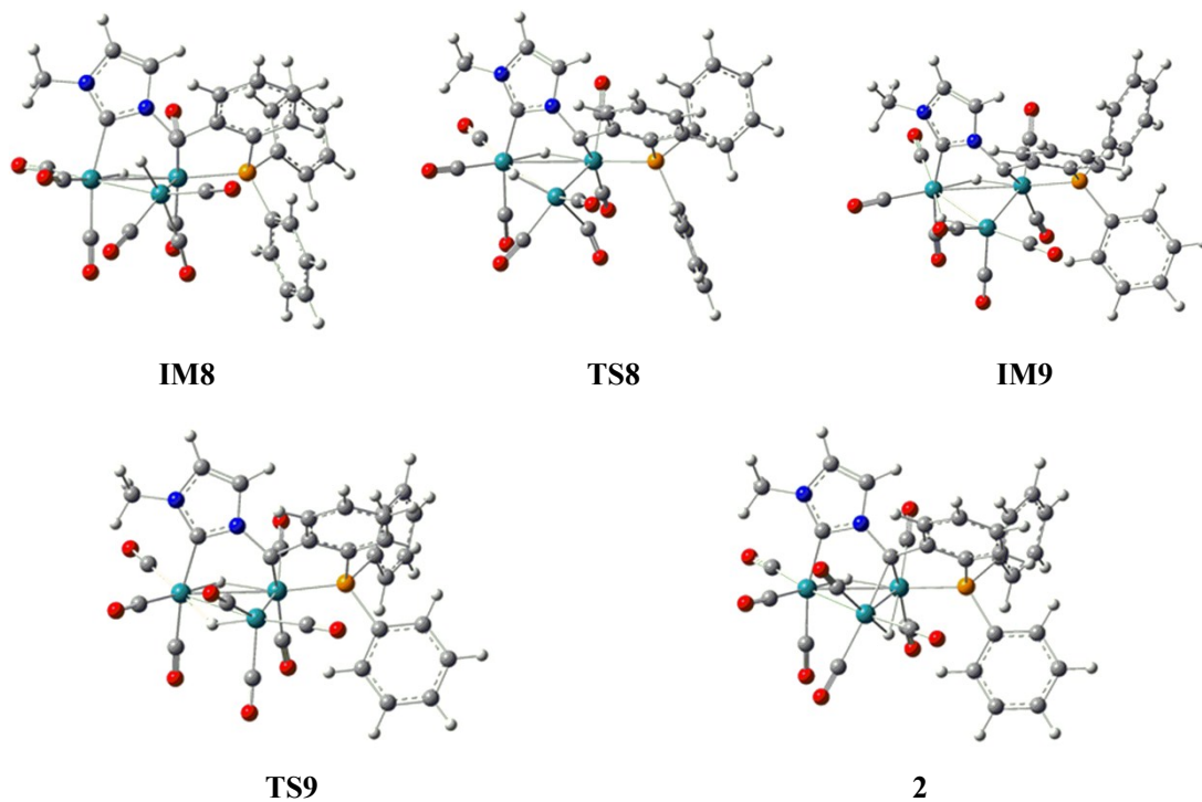
Fig. S5 Optimized geometries for the species shown in Fig. 3.
