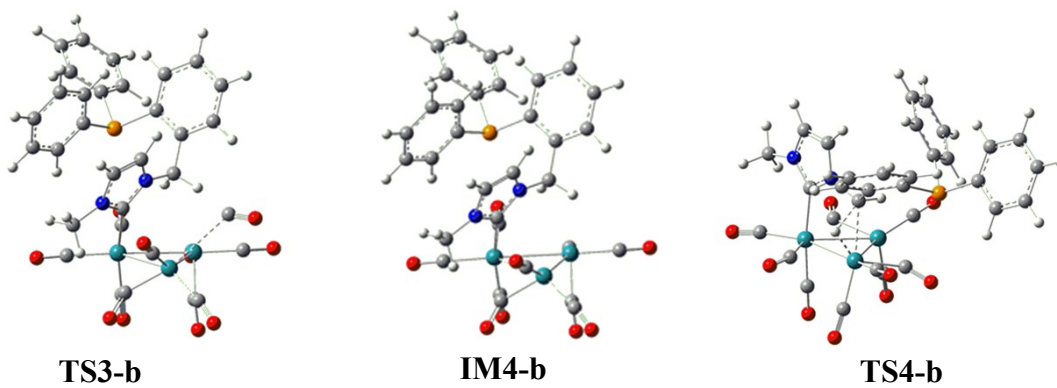
Fig. S3 Optimized geometries for the species shown in Fig. S2.
