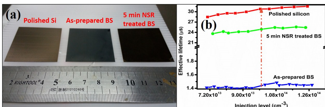
Fig.S2. (a) Typical macro pictures of different samples after ALD \text{Al}_2\text{O}_3 passivation and (b) Effective minority carrier lifetime of different samples after ALD \text{Al}_2\text{O}_3 passivation as a function of injection level.
