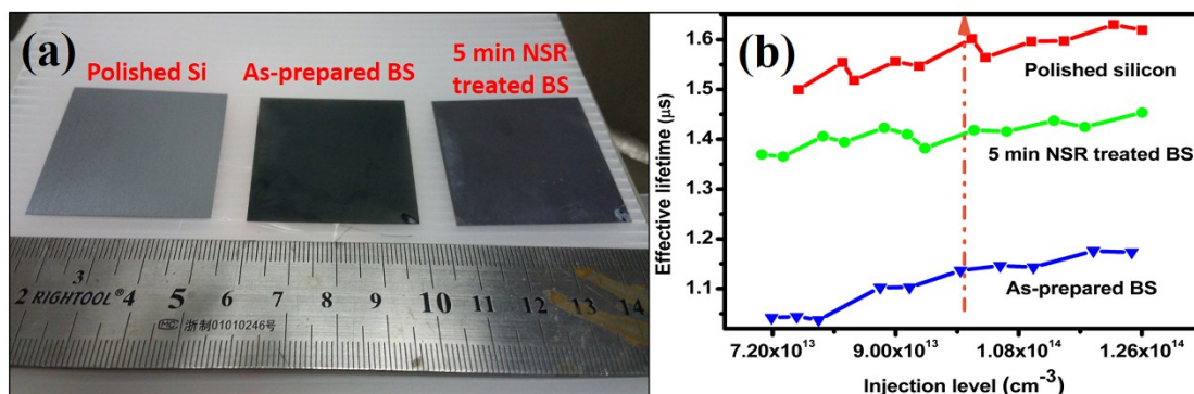
Fig.S1. (a) Typical macro pictures of different samples before ALD \text{Al}_2\text{O}_3 passivation and (b) Effective minority carrier lifetime of different samples before ALD \text{Al}_2\text{O}_3 passivation as a function of injection level.
