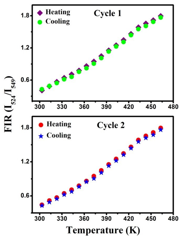
Supplementary Fig. 1 FIR vs. Temperature graph for \text{Gd}_2\text{Mo}_3\text{O}_9: 0.3\% \text{Er}^{3+}/3\% \text{Yb}^{3+} sample for two heating-cooling cycles (two heating + two cooling).
