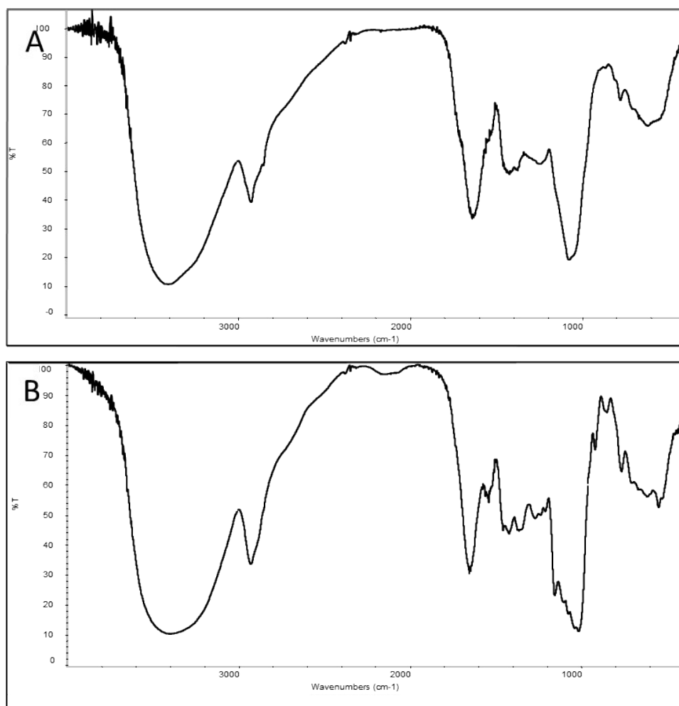
Supplementary Figure 1. FT-IR spectra of the LPI (A) and LPII (B).
