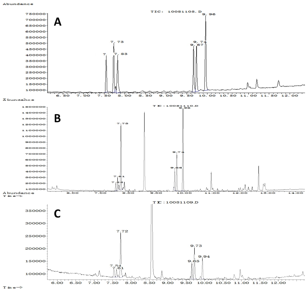
Supplementary Figure 2. GC-MS spectra of litchi polysaccharides: (A) standard sample; (B) LPI ; (C) LPII.
