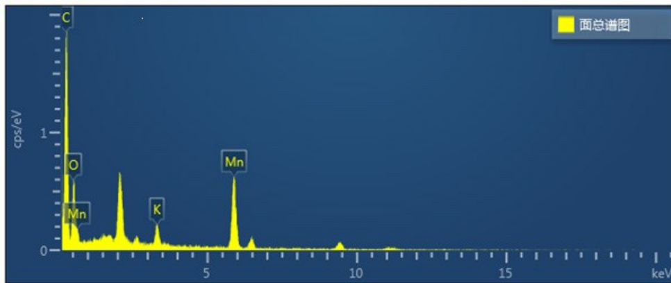
Fig. S2 EDS spectrum of RGO/MnO 2 -CNTs nanocomposites.
