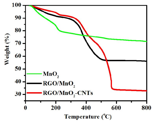
Fig. S1 TG curve of as-prepared MnO 2 , RGO/MnO 2 , and RGO/MnO 2 -CNTs
