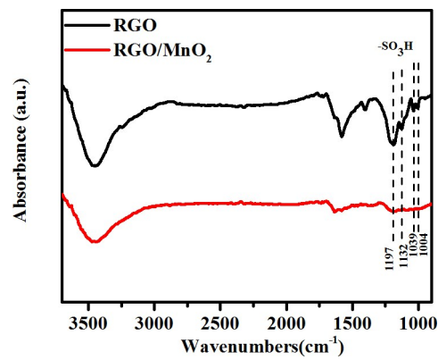
Fig. S3 FTIR spectra of RGO and RGO/MnO 2 .
