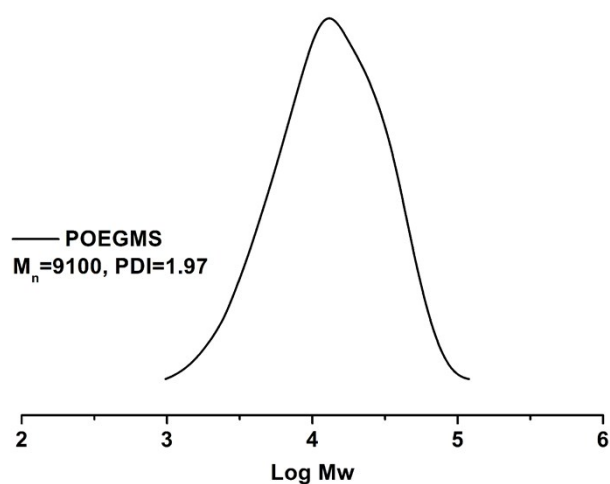
Fig. S2 GPC trace of POEGMS.
