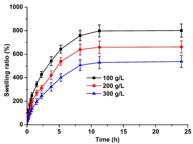
Fig. S5 Swelling curves of the lyophilized hydrogels with various original solid contents.
