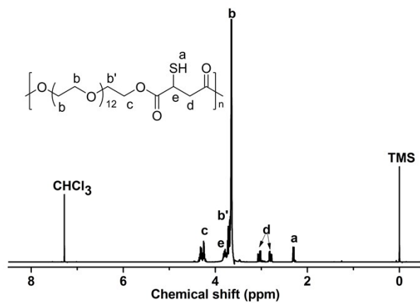
Fig. S3 ^1\text{H} NMR spectrum of POEGMS.
