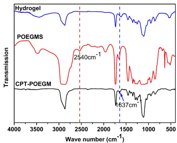
Fig. S4 FT-IR spectra of CPT-POEGM, POEGMS and hydrogel.
