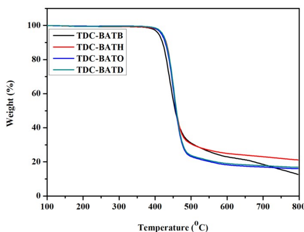
Figure S3 The TGA curves of TDC-BATB, TDC-BATH, TDC-BATO and TDC-BATD at a heating rate of 10^{\circ}\text{C}/\text{min} in \text{N}_2 .
