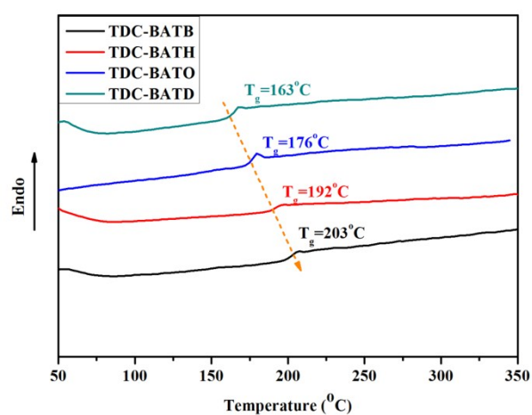
Figure S2 The DSC curves of TDC-BATB, TDC-BATH, TDC-BATO and TDC-BATD at a heating rate of 10^{\circ}\text{C}/\text{min} in \text{N}_2 .
