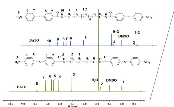
Figure S1 The ^1\text{H-NMR} spectra of monomers (BATB and BATO).
