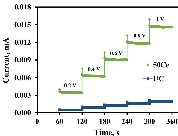
Figure S1. Chronoamperometric plot for dc conductivity measurements of uncoated (UC) and 50 cycles of CeO 2 ALD coated (50Ce) LiMn 2 O 4 particles at 25 °C.
