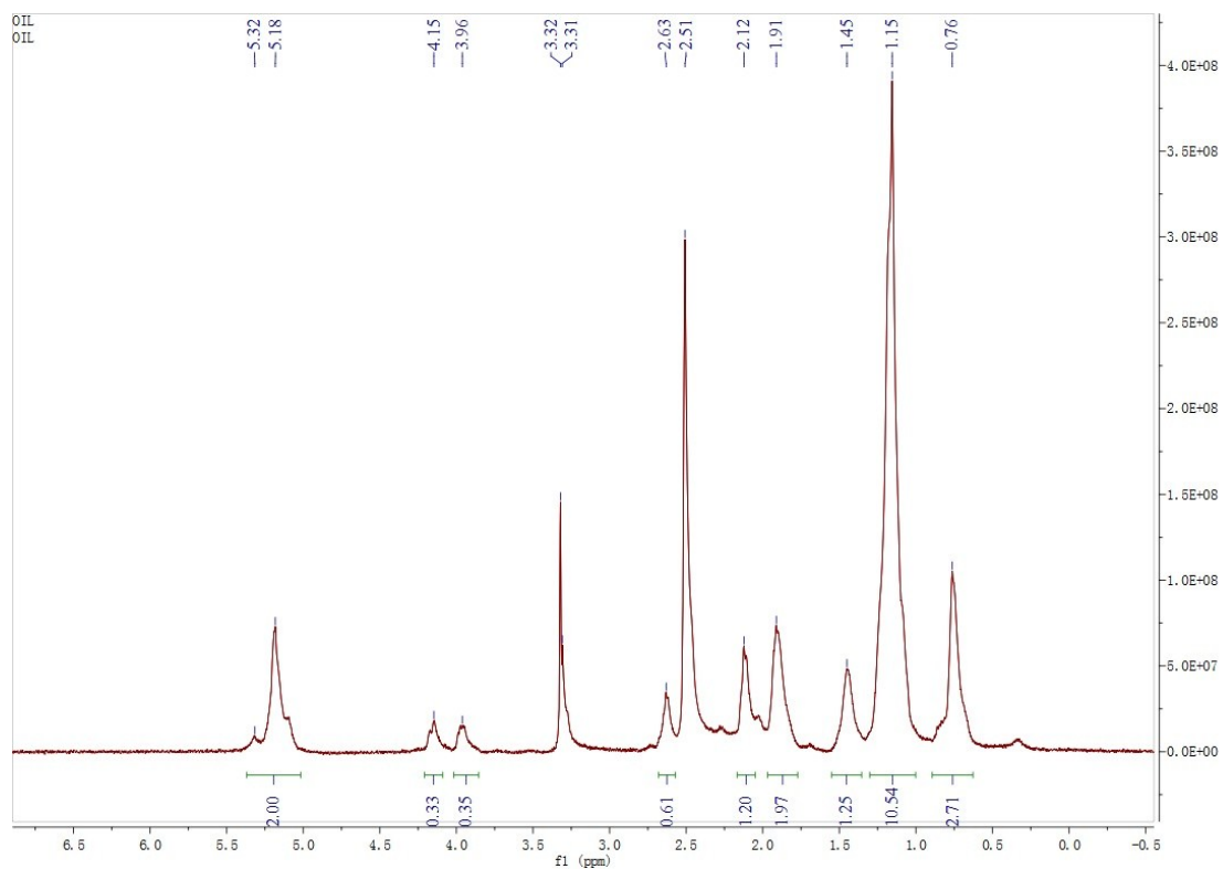
Fig. S1 1 H NMR spectra of the soybean oil
