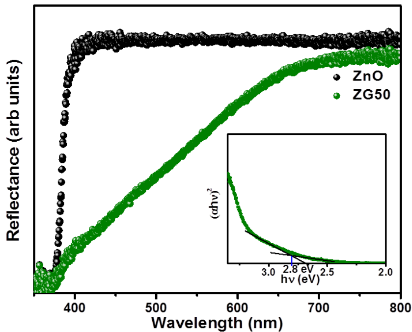
Figure 2: Diffuse reflectance spectroscopy of as prepared sample, Inset shows Tauc plot.
