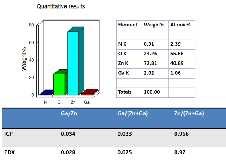
Figure 1: Elemental analysis of as prepared ZnO:GaN solid solution samples by Energy dispersive X-ray analysis (EDAX) and ICP.
