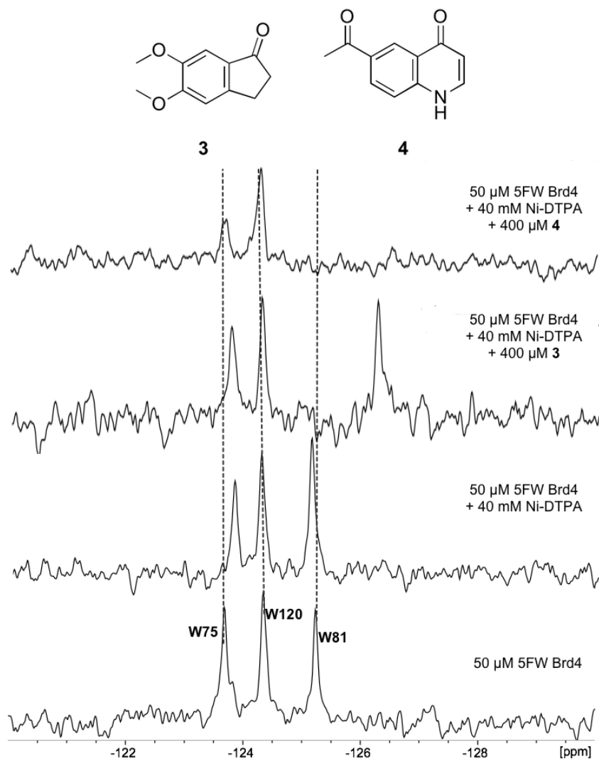
Figure S8. ProOF NMR spectra of 50 \mu M 5FW Brd4 in the presence of various fragments. Binding is evident in the presence of 20 mM Ni-DTPA for compounds 3 and 4, as shown by perturbations to the chemical shift or peakwidth of W81. Compounds 3 and 4 also bind to 5FW Brd4 in the absence of Ni-DTPA. Spectra were taken on a 600 MHz Bruker Avance III spectrometer equipped with a quadruple resonance HFCN CryoProbe without proton decoupling.
