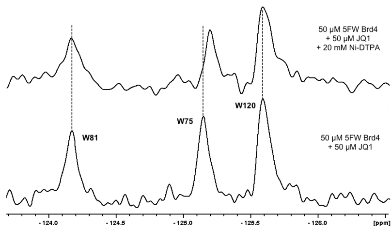
Figure S9. ProOF NMR spectra of 5FW Brd4 with (+)-JQ1 with and without Ni-DTPA. The addition of (+)-JQ1 causes W81 to move downfield of W75 and W120. The new resonance appears at the same chemical shift in the presence and absence of Ni-DTPA.
