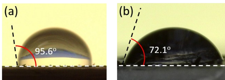
Fig. S1. Contact angle measurements of water droplets on (a) graphite and (b) MoS 2 substrates.
