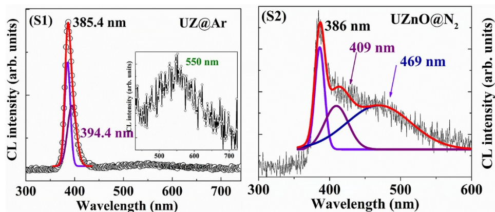
Figure S CL spectra of undoped ZnO nanostructures grown under both Ar and N 2 gas ambient.
