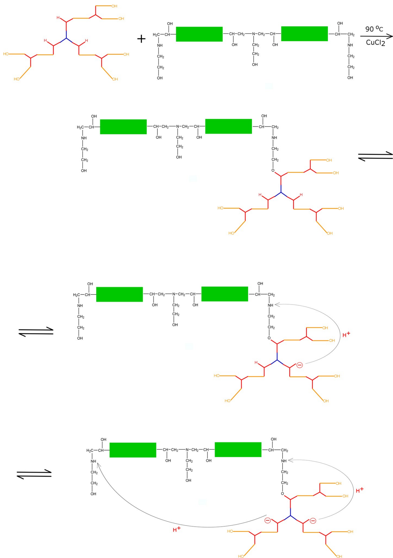
Scheme 1 – Formation of intramolecular interactions in AEBA-EM
