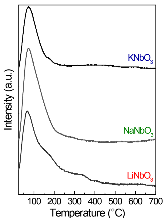
Figure S1. Oxygen desorption profiles of ANbO 3 (A=Li, Na, K) niobates.
