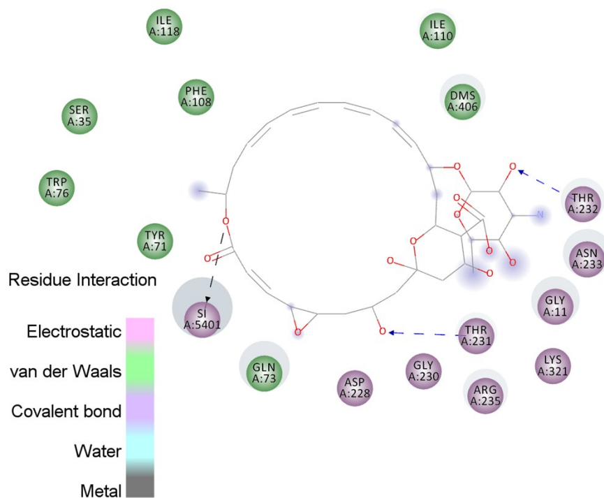
Fig. S2 Ligplot of Natamycin to BACE-1
