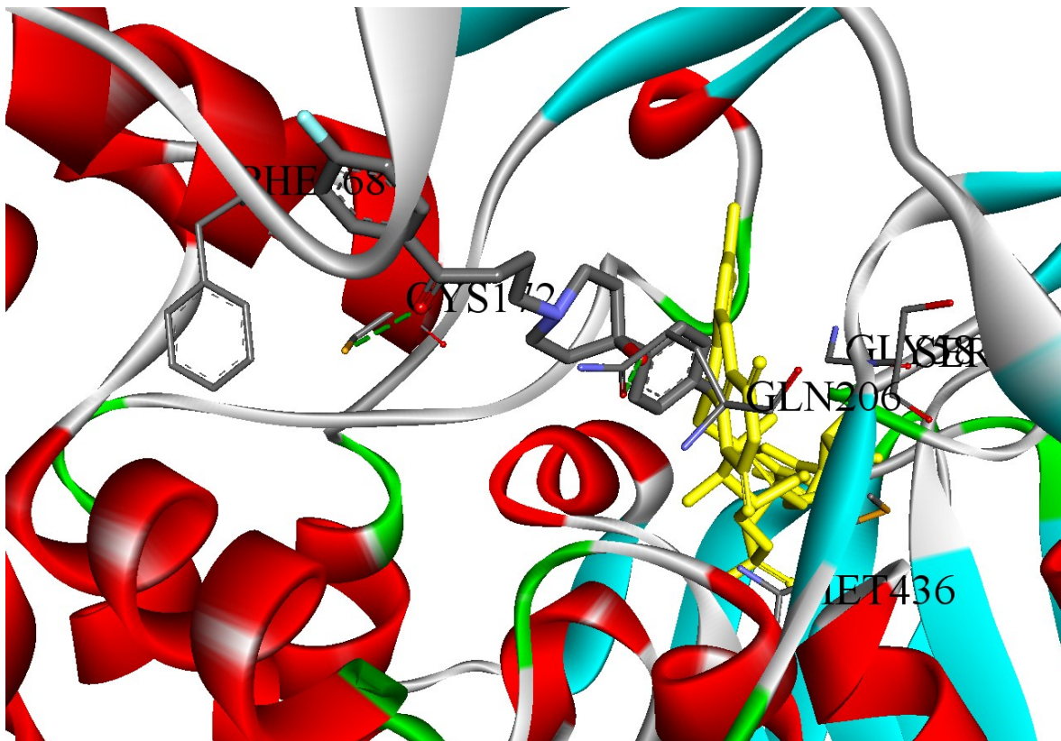
Fig. S5 The comparison of binding conformations between co-crystallized ligand of monoamine oxidase B (PDB code: 4A7A) and haloperidol
