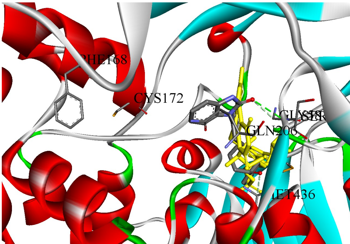
Fig. S3 The comparison of binding conformations between co-crystallized ligand of monoamine oxidase B (PDB code: 4A7A) and droperidol
