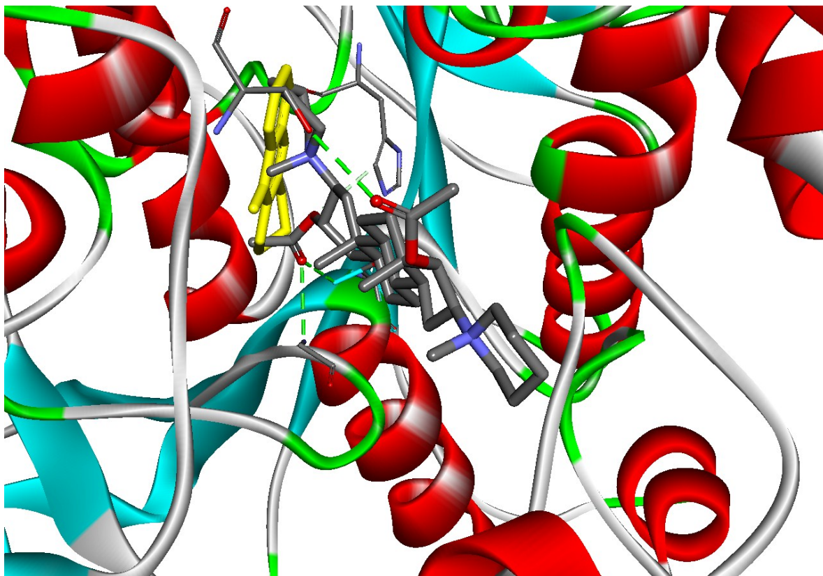
Fig. S7 The comparison of binding conformations between co-crystallized ligand of butyrylcholinesterase (PDB code: 4BDS) and pancuronium
