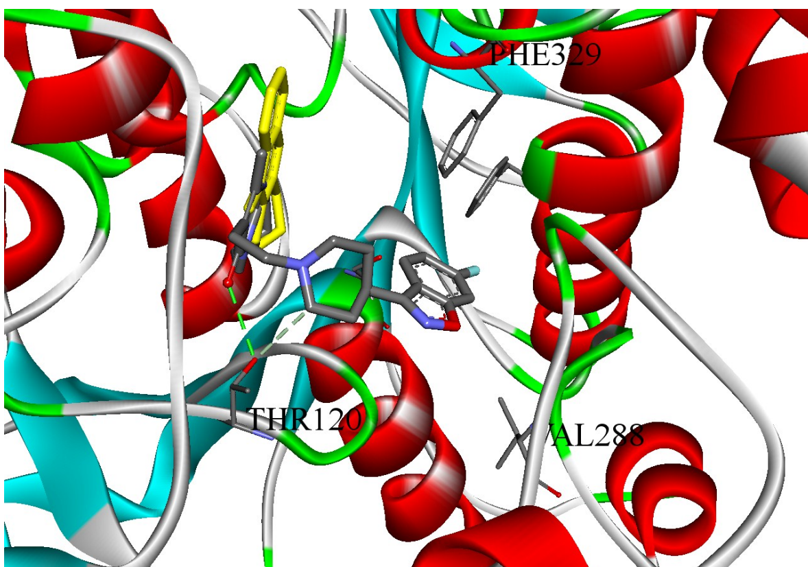
Fig. S8 The comparison of binding conformations between co-crystallized ligand of butyrylcholinesterase (PDB code: 4BDS) and risperidone
