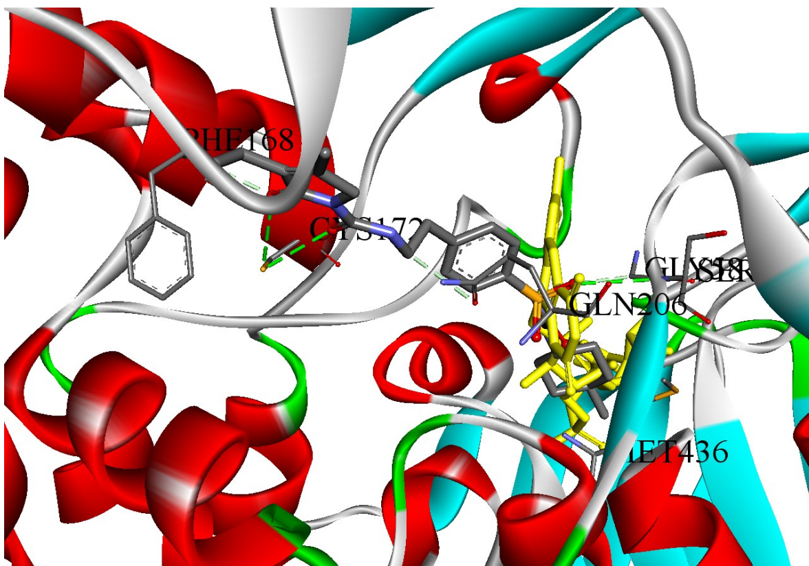
Fig. S4 The comparison of binding conformations between co-crystallized ligand of monoamine oxidase B (PDB code: 4A7A) and glimepiride
