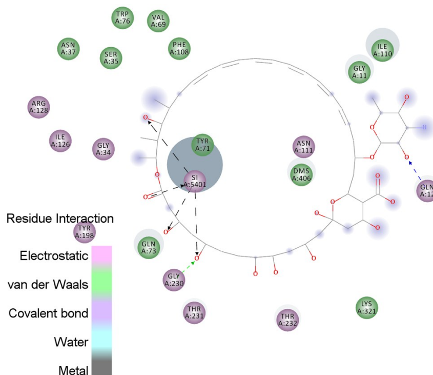
Fig. S1 Ligplot of Amphotericin B to BACE-1
