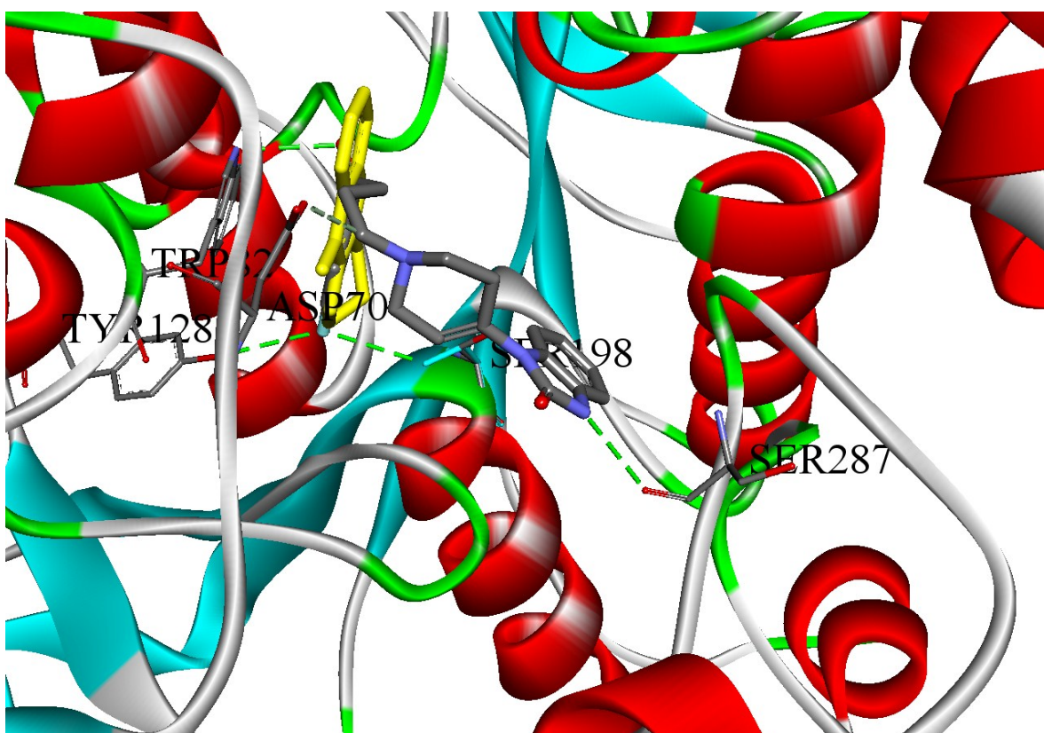
Fig. S6 The comparison of binding conformations between co-crystallized ligand of butyrylcholinesterase (PDB code: 4BDS) and droperidol
