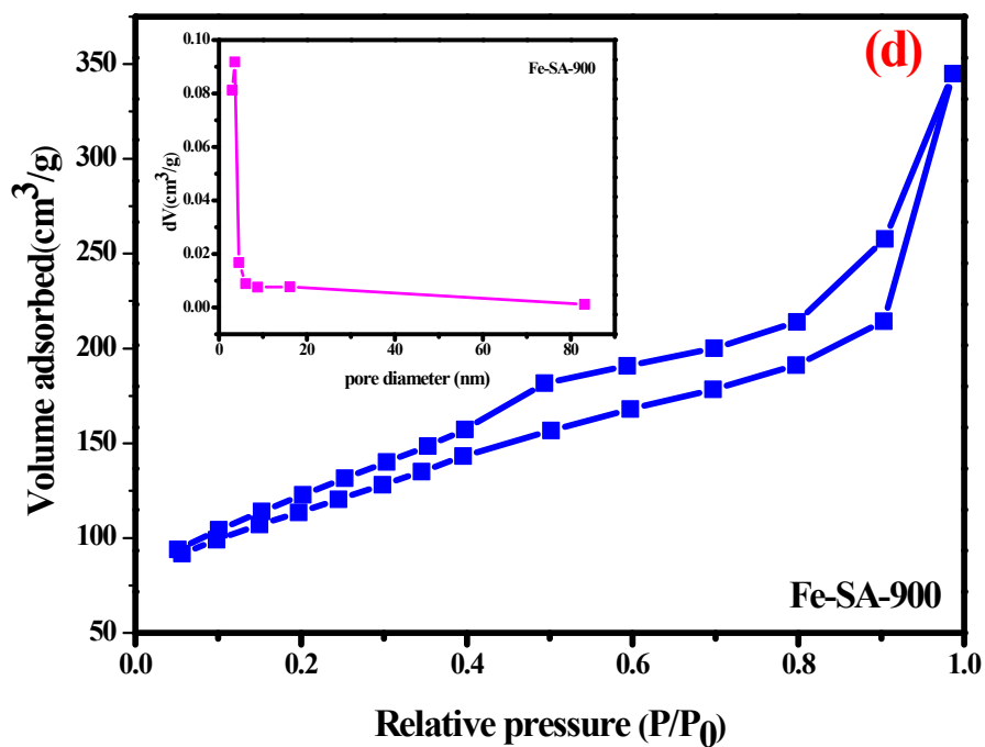
Fig. S1 The BET of (a)Fe-SA-600, (b)Fe-SA-700, (c)Fe-SA-800, and (d) Fe-SA-900.
