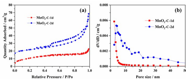
Fig. S1 (a) N_2 adsorption-desorption isotherms and (b) BJH pore size distribution plots for MoO_2-C-1d and MoO_2-C-2d .
