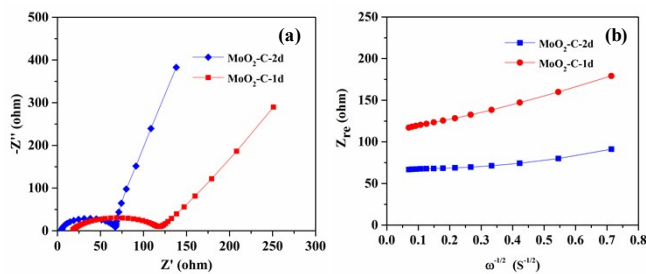
Fig. S2 (a) Nyquist plots and (b) the relationship between Z_{re} and \omega^{-1/2} for the MoO_2-C-1d and MoO_2-C-2d electrodes after 50 cycles from 1 MHz to 0.05 Hz.
