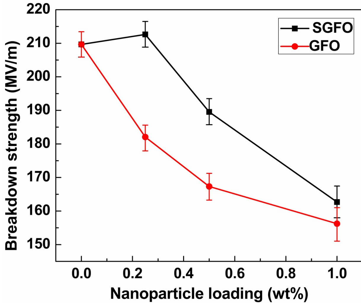
Fig. S2 Variation of breakdown strength GFO-PVDF composites and SGFO-PVDF composites.
