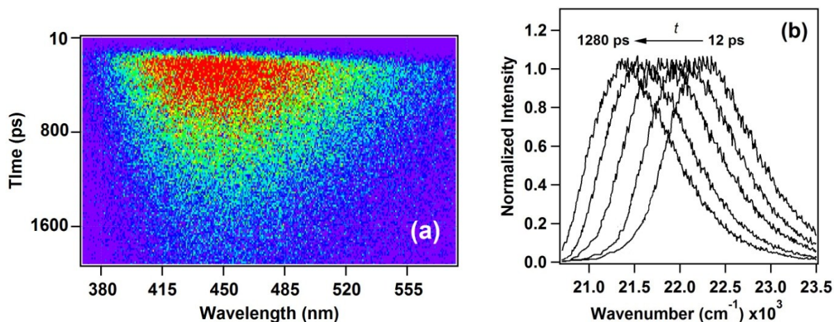
Figure S1. (a) The streak camera data and (b) time-resolved emission spectra (TRES) of C480 in PtOH-CHCl 3 binary solvent mixture.
