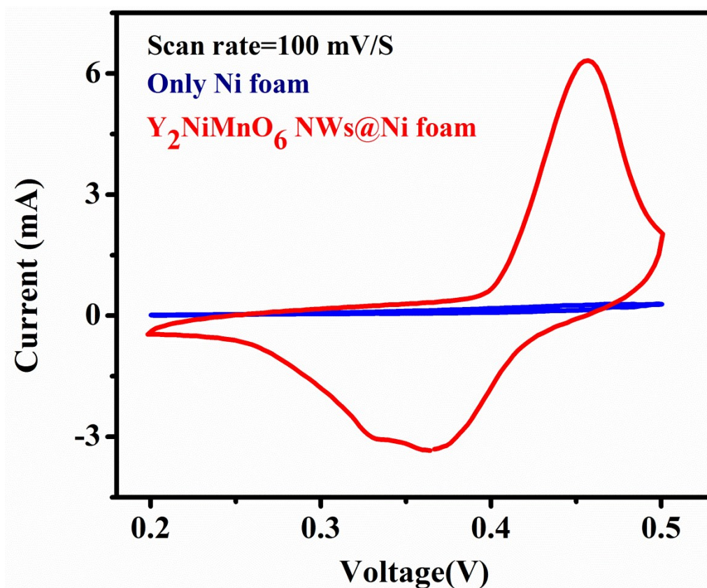
Figure S2: Comparison between the CV curves of only Ni foam and \text{Y}_2\text{NiMnO}_6 NWs over Ni foam at scan rate of 100 \text{ mV s}^{-1} .
