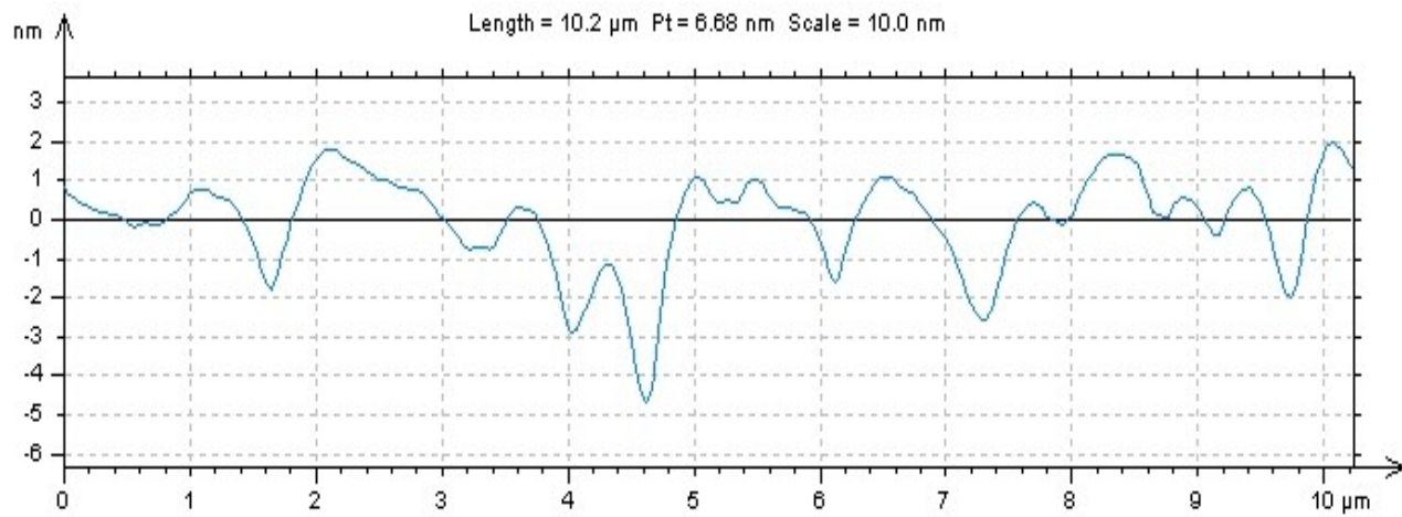
Fig.S3. AFM surface roughness profile for (a) Pristine SPPEK and (b) SPPEK-SGNF (0.5 wt.%).
