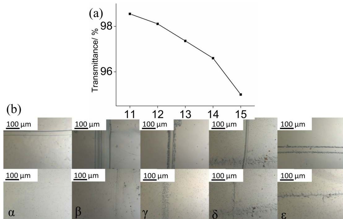
Figure S4. (a) Transparency property and (b) self-healing property of the (CS/DF-PEG) 15 film undergoing eleventh to fifteenth damage/healing process
