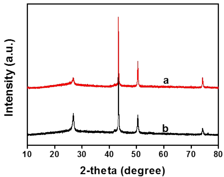
Figure S3. XRD patterns of 29.4 wt % Cu/BN catalyst (a) before and (b) after the reaction of hydrolysis of AB.
