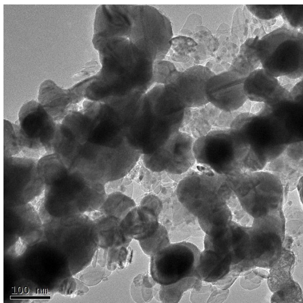
Figure S2. TEM image of 29.4 wt % Cu/ h -BN catalyst after the hydrolytic reaction of AB.
