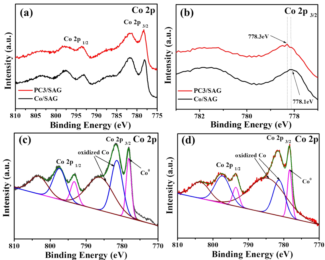
Fig. S1. (a) XPS spectra of Co 2p for Co/SAG and PC3/SAG. (b) Comparison of the Co 2p 3/2 from Co/SAG and PC3/SAG. Deconvoluted Co-2p X-ray photoelectron spectra for (c) Co/SAG and (d) PC3/SAG.
