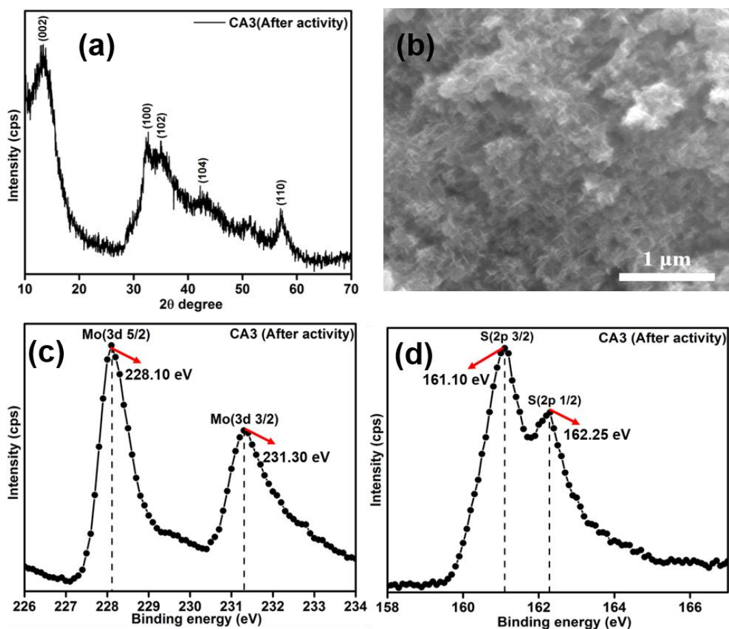
Fig. S1. XRD spectra (a), FESEM (c) and XPS spectra of (c) Mo 3d state, (d) S
