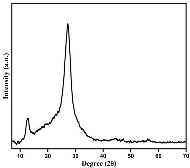
Figure S1: XRD patterns of gC 3 N 4
