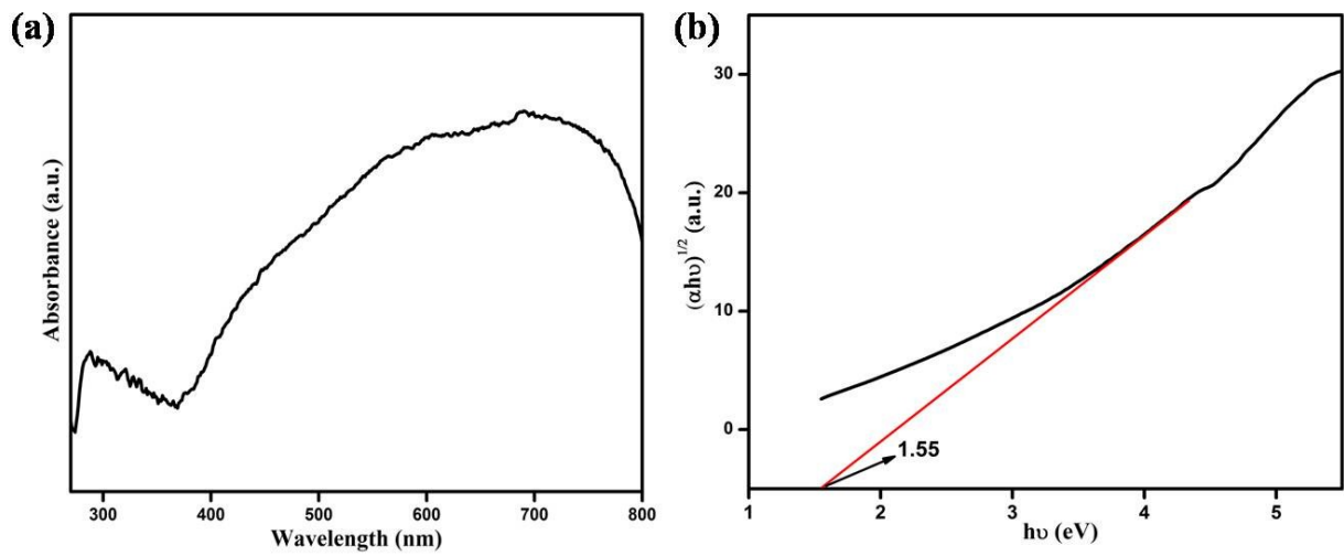
Figure S3: UV-Visible absorption spectra (a) and calculated band gap (b) of CuO
