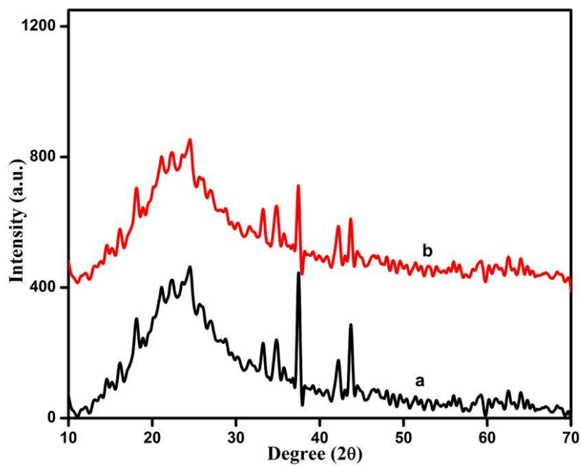
Figure S2: XRD patterns of CCM-4 (a) and CCM-4 after 5 runs (b)
