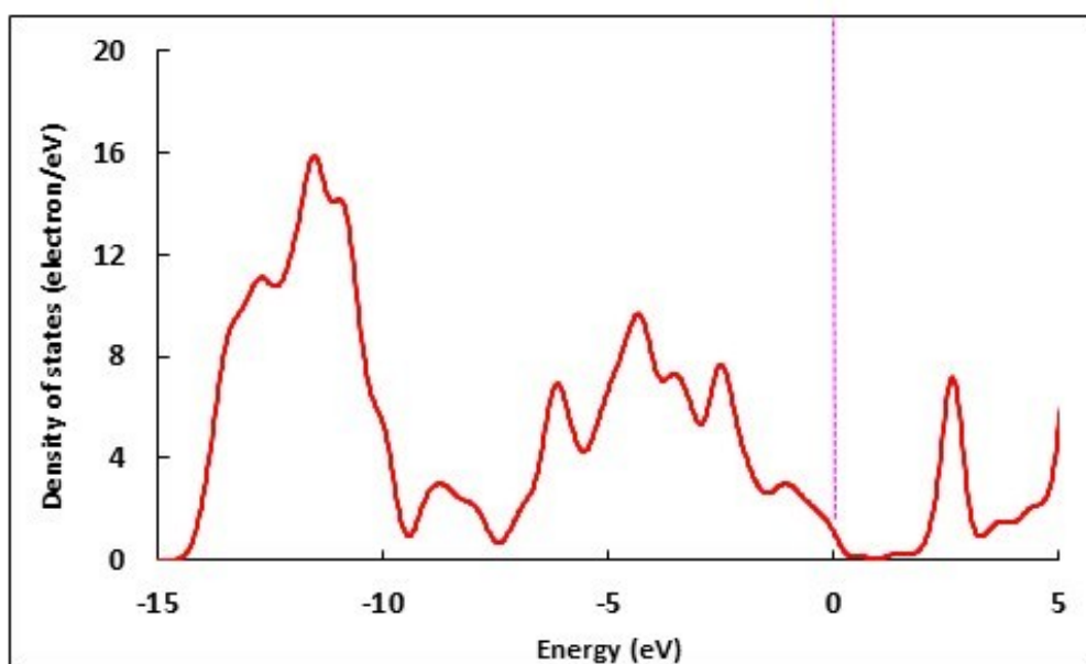
S2. Total density of states of CuCo-oxide ( \text{CoCu}_2\text{O}_3 ) clusters.
