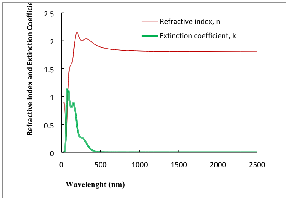
S5. Refractive index ( n ) and extinction coefficient ( k ) spectra of CuCo-oxide coatings.
