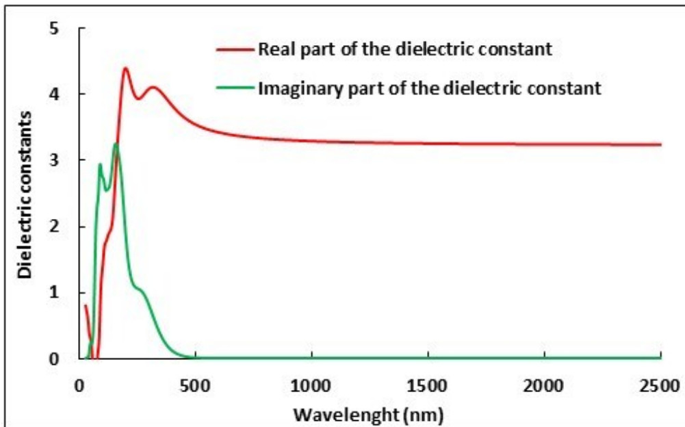
S4. Real and imaginary parts of dielectric constants of CoCu 2 O 3 clusters.
