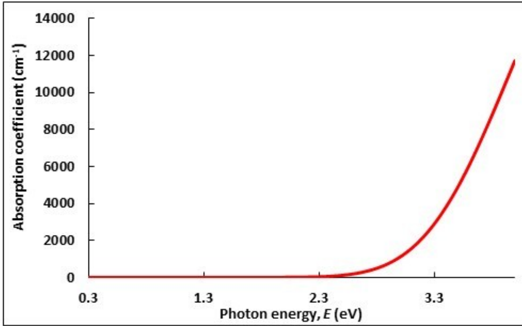
S3. Theoretical absorption spectrum of CoCu 2 O 3 clusters
