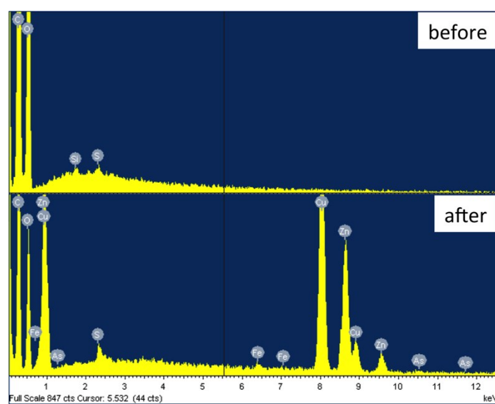
Figure S1: EDS images of membranes, before and after adsorption
