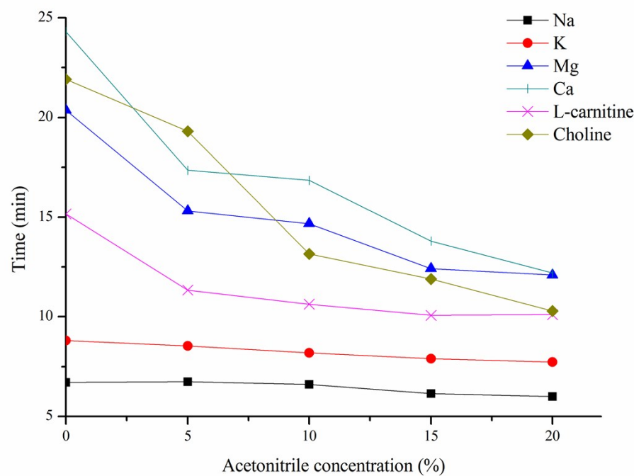
Fig. S2 The ratio of acetonitrile on the separation performance of analytical column
