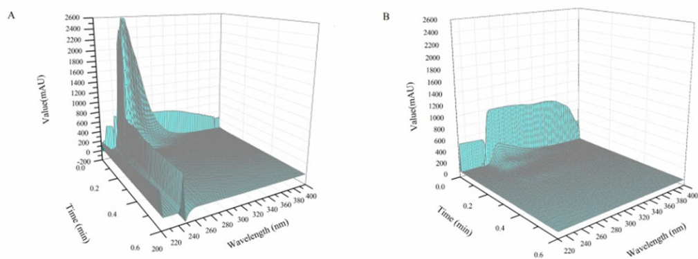
Fig. S1 Three dimensional diagram of the real sample, analysis of milk sample by direct injection at the flow rate of 1 \text{ mL min}^{-1} (A), 1 \text{ mL min}^{-1} (B).
